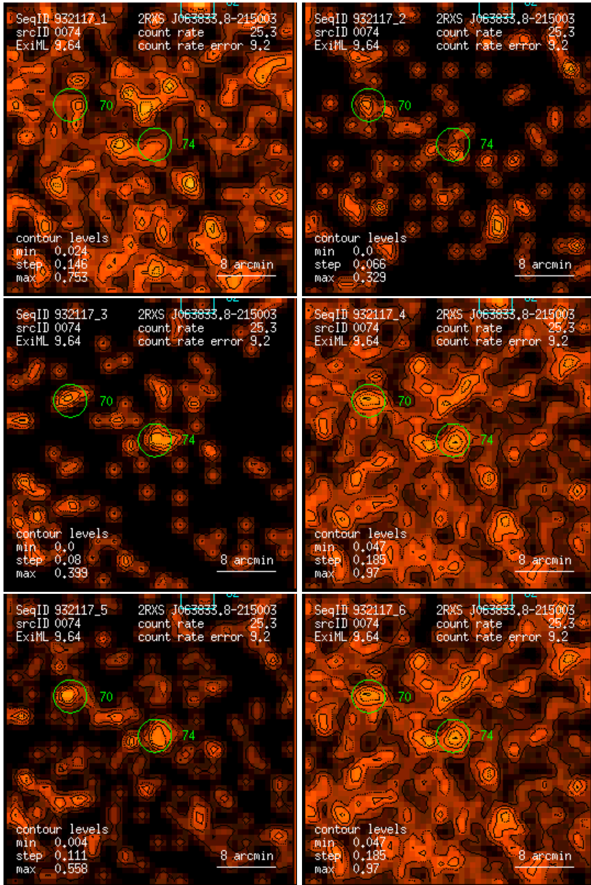
Figure 74: RASS 932117: detection 0074: band rate images, Gaussian filter: (1) PSPC channels 11 – 41, (2) 52 – 90, (3) 91 – 201, (4) 11 – 235, (5) 52 – 201, (6) 11 – 201. Broad band rates in counts/ks. Band rate contour levels in counts/ks/arcmin 2 .
