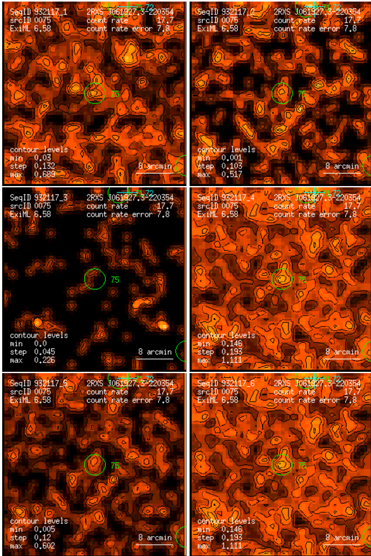
Figure 75: RASS 932117: detection 0075: band rate images, Gaussian filter: (1) PSPC channels 11 – 41, (2) 52 – 90, (3) 91 – 201, (4) 11 – 235, (5) 52 – 201, (6) 11 – 201. Broad band rates in counts/ks. Band rate contour levels in counts/ks/arcmin 2 .
