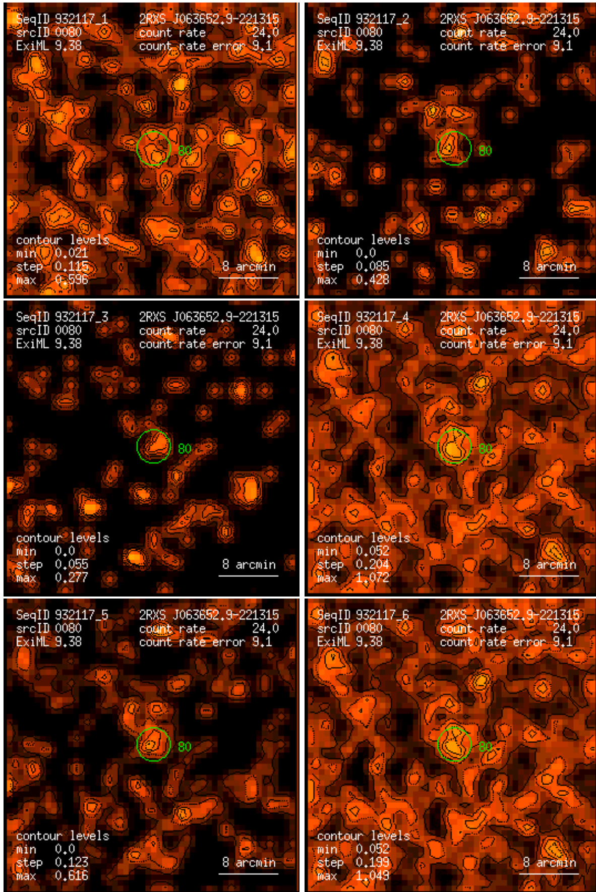
Figure 80: RASS 932117: detection 0080: band rate images, Gaussian filter: (1) PSPC channels 11 – 41, (2) 52 – 90, (3) 91 – 201, (4) 11 – 235, (5) 52 – 201, (6) 11 – 201. Broad band rates in counts/ks. Band rate contour levels in counts/ks/arcmin 2 .
