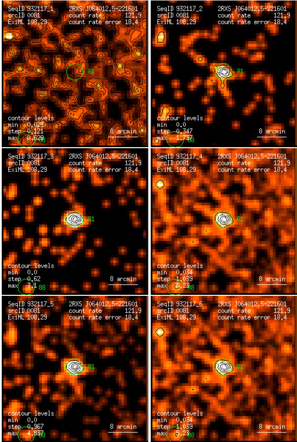
Figure 81: RASS 932117: detection 0081: band rate images, Gaussian filter: (1) PSPC channels 11 – 41, (2) 52 – 90, (3) 91 – 201, (4) 11 – 235, (5) 52 – 201, (6) 11 – 201. Broad band rates in counts/ks. Band rate contour levels in counts/ks/arcmin 2 .
