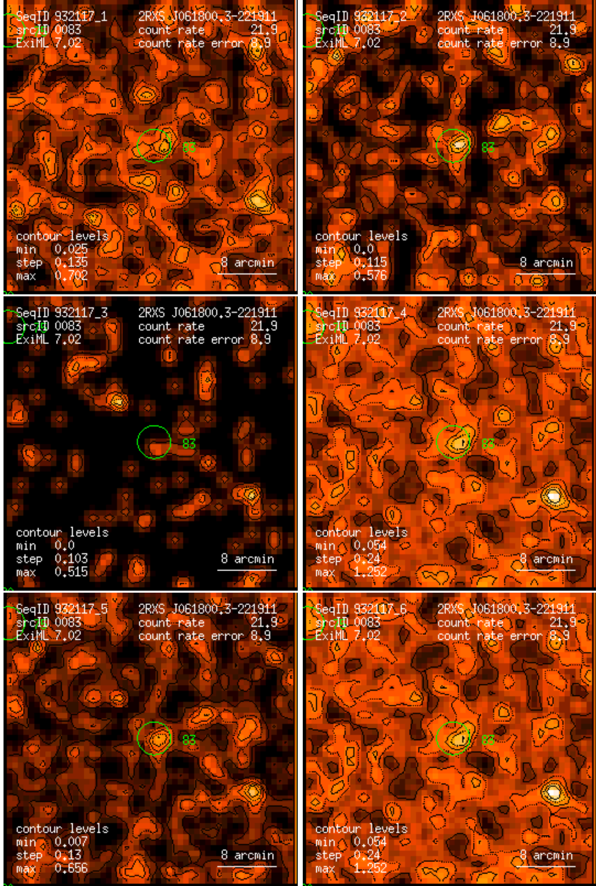
Figure 83: RASS 932117: detection 0083: band rate images, Gaussian filter: (1) PSPC channels 11 – 41, (2) 52 – 90, (3) 91 – 201, (4) 11 – 235, (5) 52 – 201, (6) 11 – 201. Broad band rates in counts/ks. Band rate contour levels in counts/ks/arcmin 2 .
