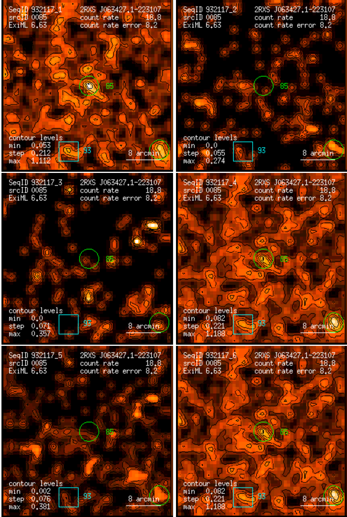
Figure 85: RASS 932117: detection 0085: band rate images, Gaussian filter: (1) PSPC channels 11 – 41, (2) 52 – 90, (3) 91 – 201, (4) 11 – 235, (5) 52 – 201, (6) 11 – 201. Broad band rates in counts/ks. Band rate contour levels in counts/ks/arcmin 2 .
