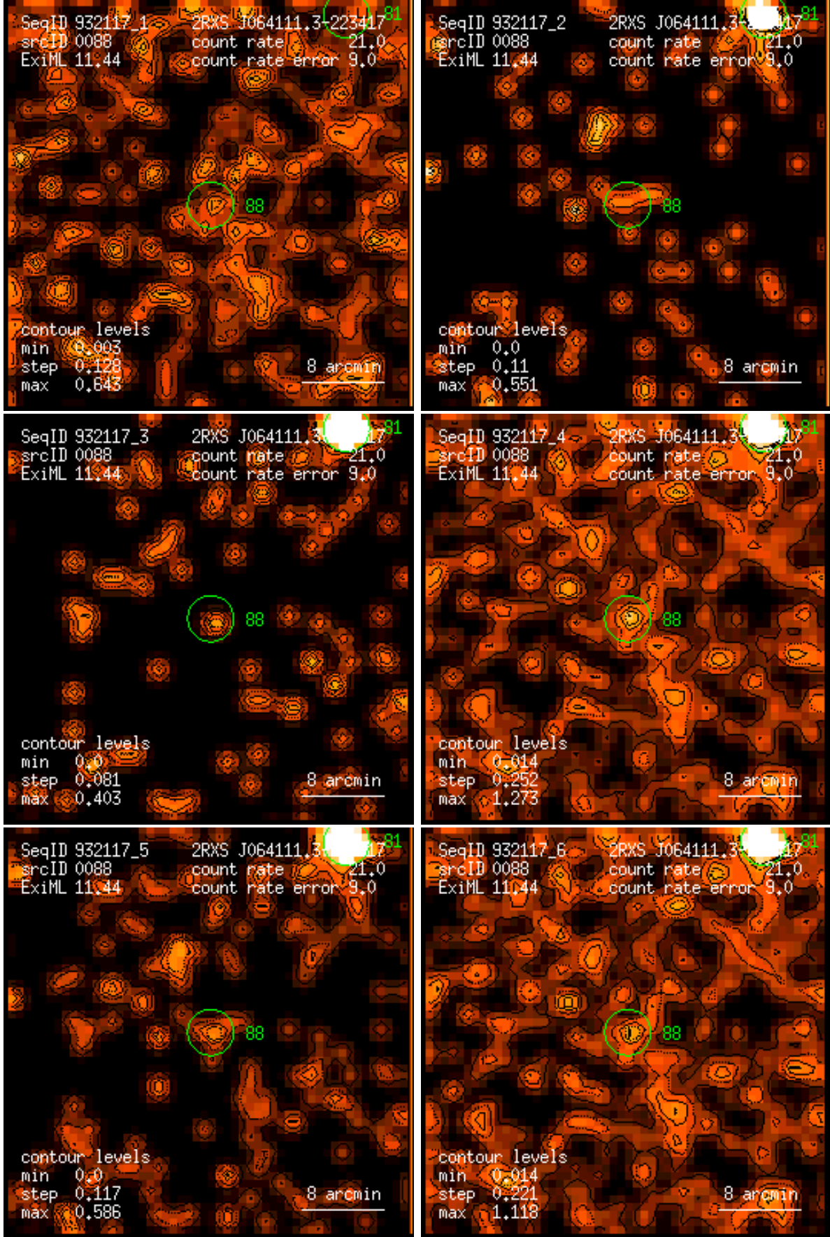
Figure 88: RASS 932117: detection 0088: band rate images, Gaussian filter: (1) PSPC channels 11 – 41, (2) 52 – 90, (3) 91 – 201, (4) 11 – 235, (5) 52 – 201, (6) 11 – 201. Broad band rates in counts/ks. Band rate contour levels in counts/ks/arcmin 2 .
