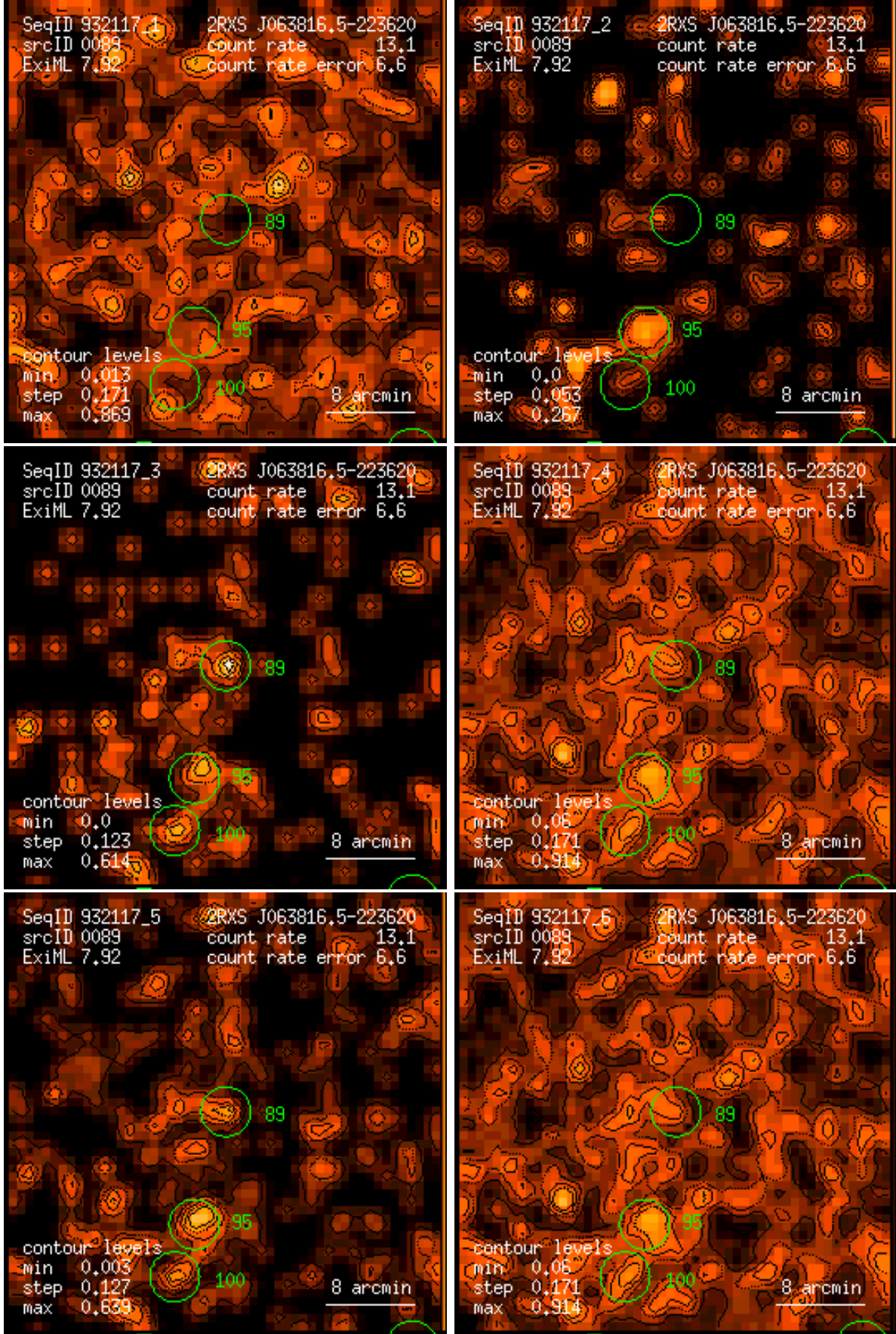
Figure 89: RASS 932117: detection 0089: band rate images, Gaussian filter: (1) PSPC channels 11 – 41, (2) 52 – 90, (3) 91 – 201, (4) 11 – 235, (5) 52 – 201, (6) 11 – 201. Broad band rates in counts/ks. Band rate contour levels in counts/ks/arcmin 2 .
