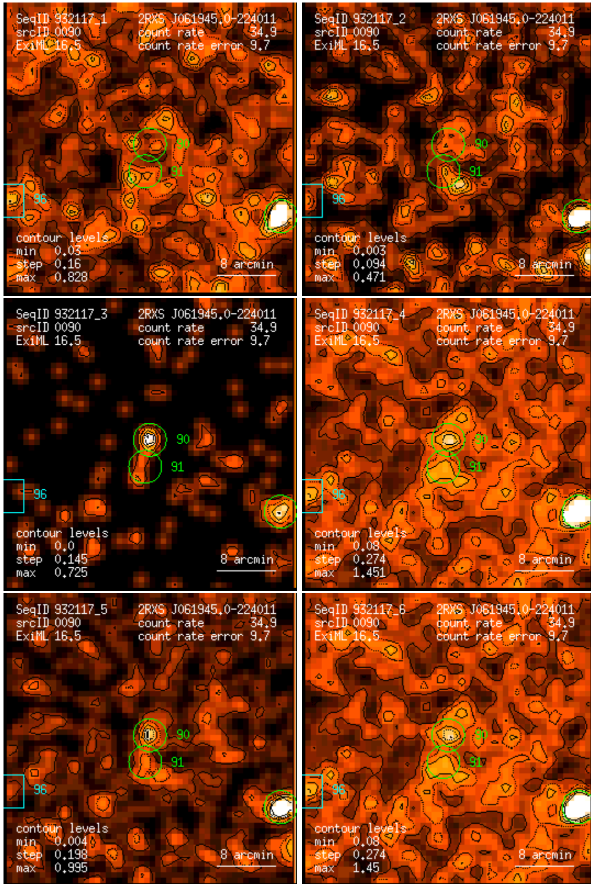
Figure 90: RASS 932117: detection 0090: band rate images, Gaussian filter: (1) PSPC channels 11 – 41, (2) 52 – 90, (3) 91 – 201, (4) 11 – 235, (5) 52 – 201, (6) 11 – 201. Broad band rates in counts/ks. Band rate contour levels in counts/ks/arcmin 2 .
