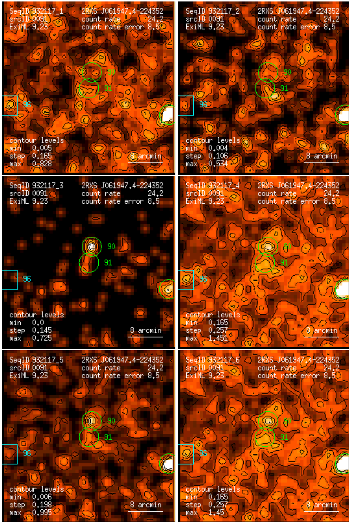
Figure 91: RASS 932117: detection 0091: band rate images, Gaussian filter: (1) PSPC channels 11 – 41, (2) 52 – 90, (3) 91 – 201, (4) 11 – 235, (5) 52 – 201, (6) 11 – 201. Broad band rates in counts/ks. Band rate contour levels in counts/ks/arcmin 2 .
