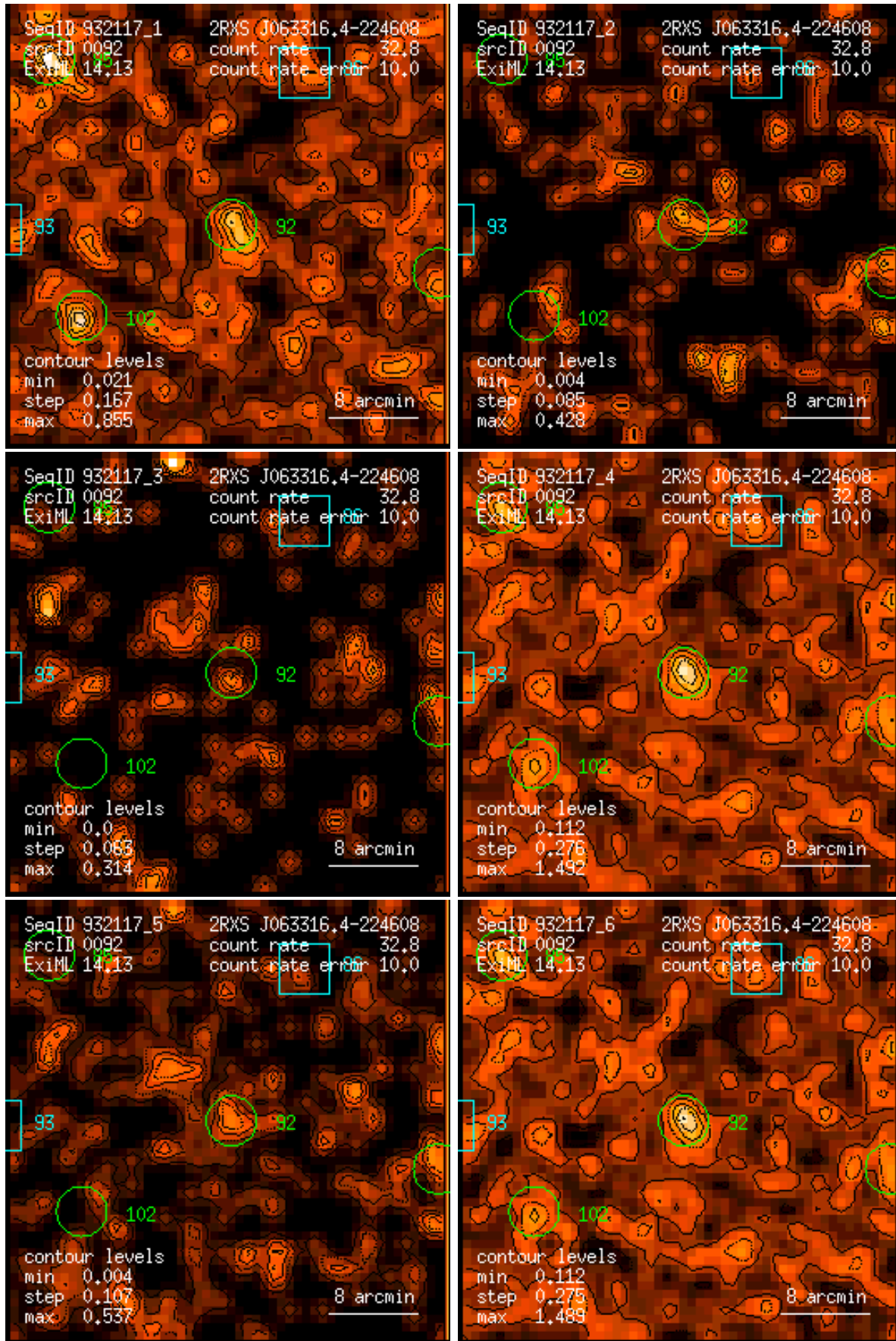
Figure 92: RASS 932117: detection 0092: band rate images, Gaussian filter: (1) PSPC channels 11 – 41, (2) 52 – 90, (3) 91 – 201, (4) 11 – 235, (5) 52 – 201, (6) 11 – 201. Broad band rates in counts/ks. Band rate contour levels in counts/ks/arcmin 2 .
