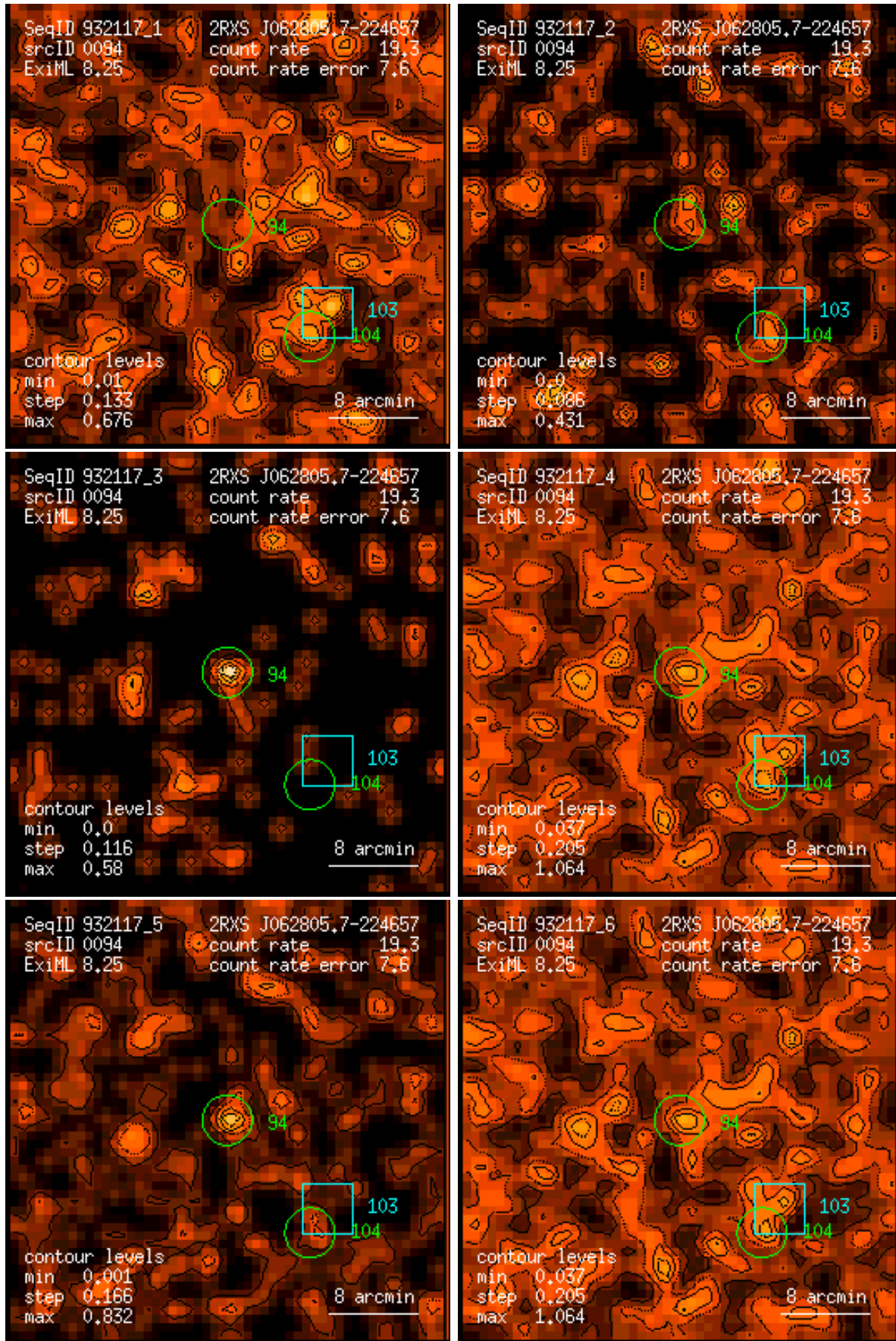
Figure 94: RASS 932117: detection 0094: band rate images, Gaussian filter: (1) PSPC channels 11 – 41, (2) 52 – 90, (3) 91 – 201, (4) 11 – 235, (5) 52 – 201, (6) 11 – 201. Broad band rates in counts/ks. Band rate contour levels in counts/ks/arcmin 2 .
