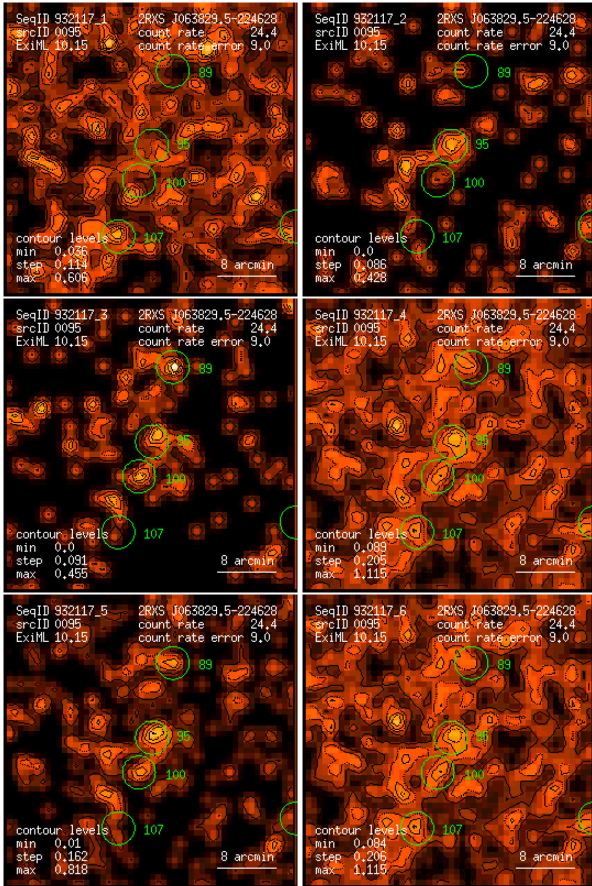
Figure 95: RASS 932117: detection 0095: band rate images, Gaussian filter: (1) PSPC channels 11 – 41, (2) 52 – 90, (3) 91 – 201, (4) 11 – 235, (5) 52 – 201, (6) 11 – 201. Broad band rates in counts/ks. Band rate contour levels in counts/ks/arcmin 2 .
