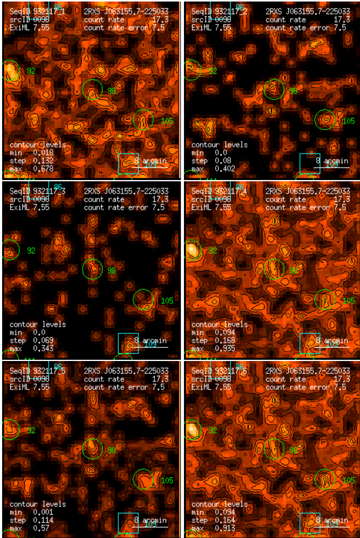
Figure 98: RASS 932117: detection 0098: band rate images, Gaussian filter: (1) PSPC channels 11 – 41, (2) 52 – 90, (3) 91 – 201, (4) 11 – 235, (5) 52 – 201, (6) 11 – 201. Broad band rates in counts/ks. Band rate contour levels in counts/ks/arcmin 2 .
