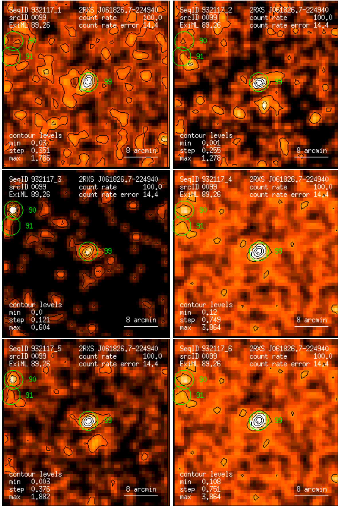
Figure 99: RASS 932117: detection 0099: band rate images, Gaussian filter: (1) PSPC channels 11 – 41, (2) 52 – 90, (3) 91 – 201, (4) 11 – 235, (5) 52 – 201, (6) 11 – 201. Broad band rates in counts/ks. Band rate contour levels in counts/ks/arcmin 2 .
