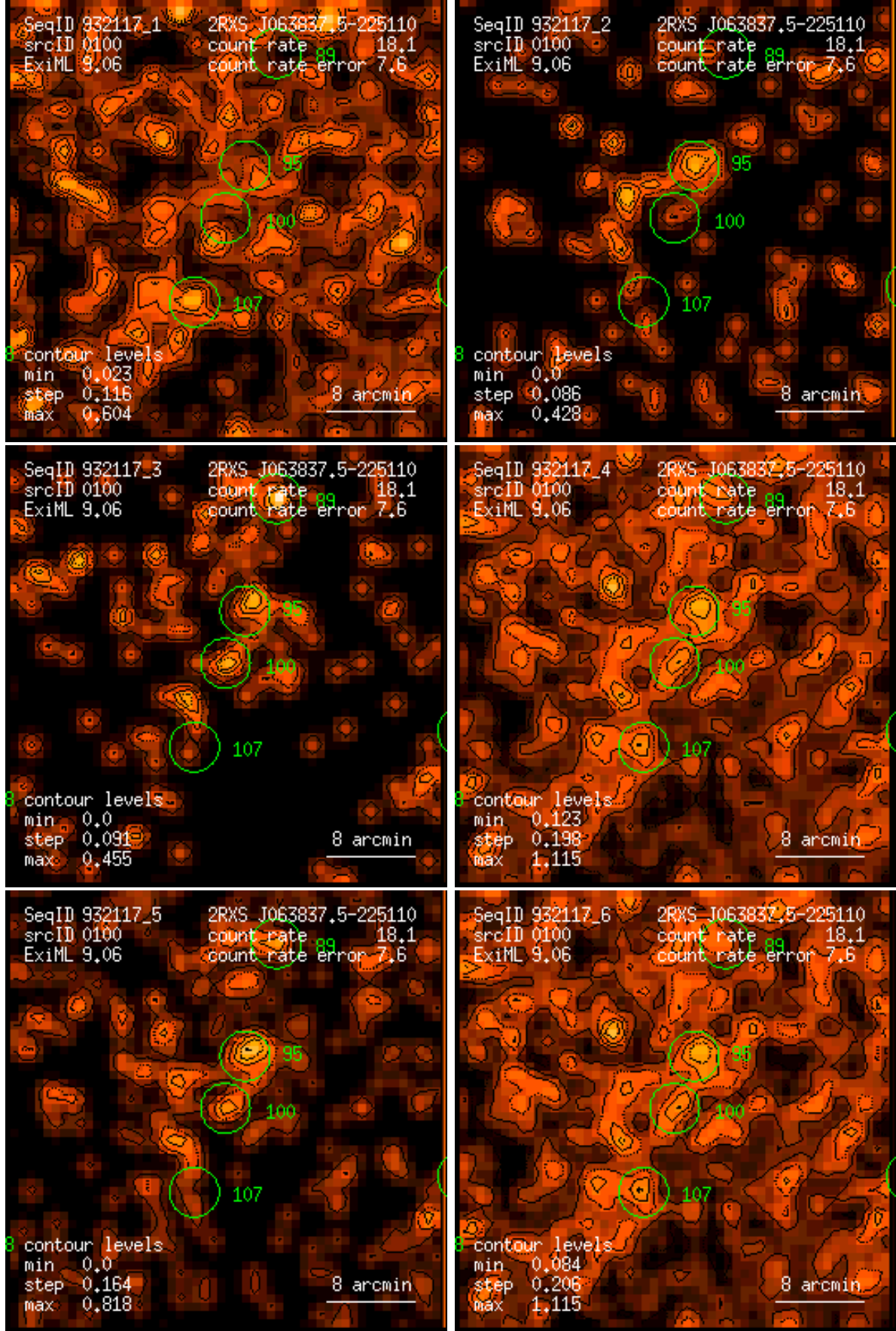
Figure 100: RASS 932117: detection 0100: band rate images, Gaussian filter: (1) PSPC channels 11 – 41, (2) 52 – 90, (3) 91 – 201, (4) 11 – 235, (5) 52 – 201, (6) 11 – 201. Broad band rates in counts/ks. Band rate contour levels in counts/ks/arcmin 2 .
