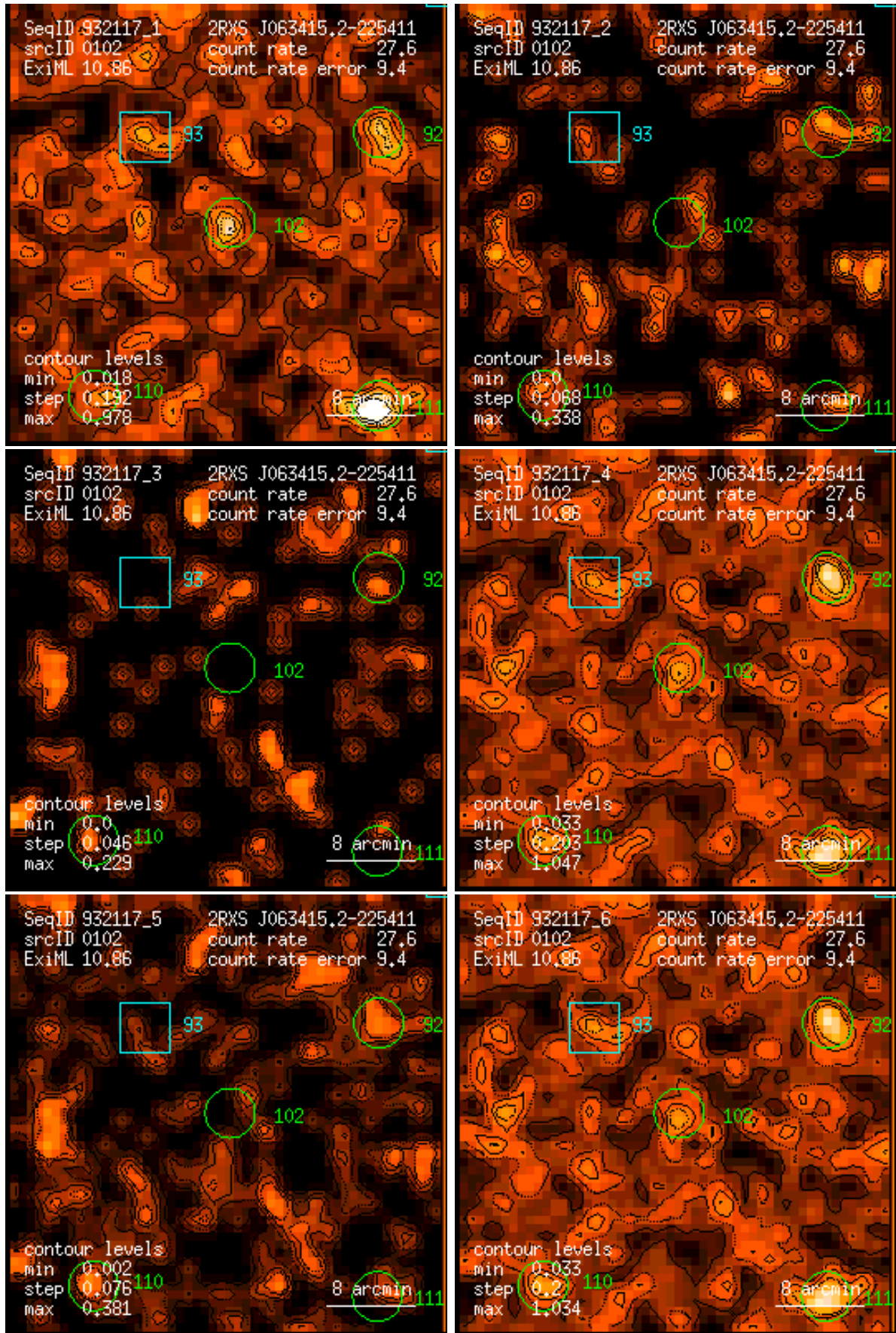
Figure 102: RASS 932117: detection 0102: band rate images, Gaussian filter: (1) PSPC channels 11 – 41, (2) 52 – 90, (3) 91 – 201, (4) 11 – 235, (5) 52 – 201, (6) 11 – 201. Broad band rates in counts/ks. Band rate contour levels in counts/ks/arcmin 2 .
