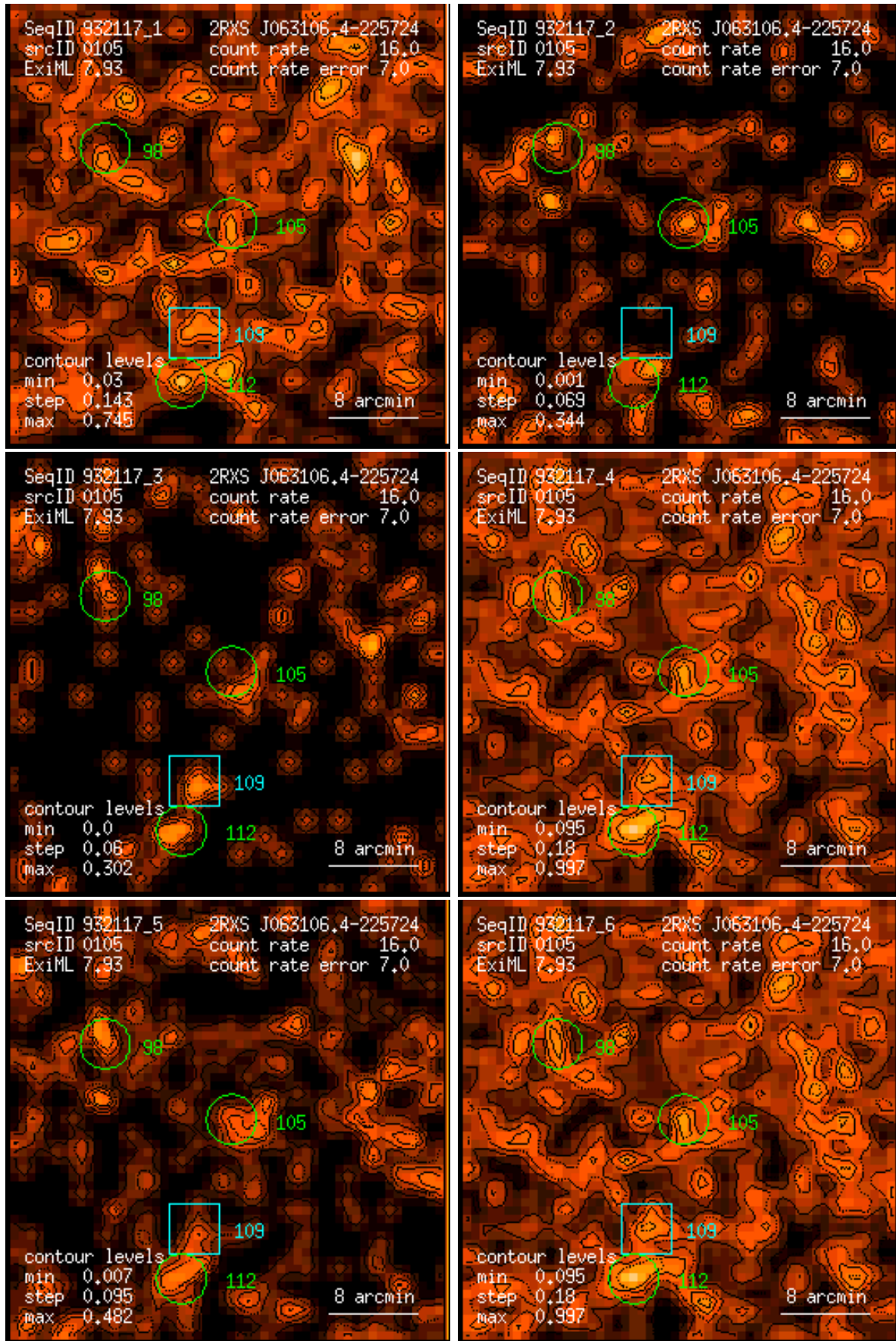
Figure 105: RASS 932117: detection 0105: band rate images, Gaussian filter: (1) PSPC channels 11 – 41, (2) 52 – 90, (3) 91 – 201, (4) 11 – 235, (5) 52 – 201, (6) 11 – 201. Broad band rates in counts/ks. Band rate contour levels in counts/ks/arcmin 2 .
