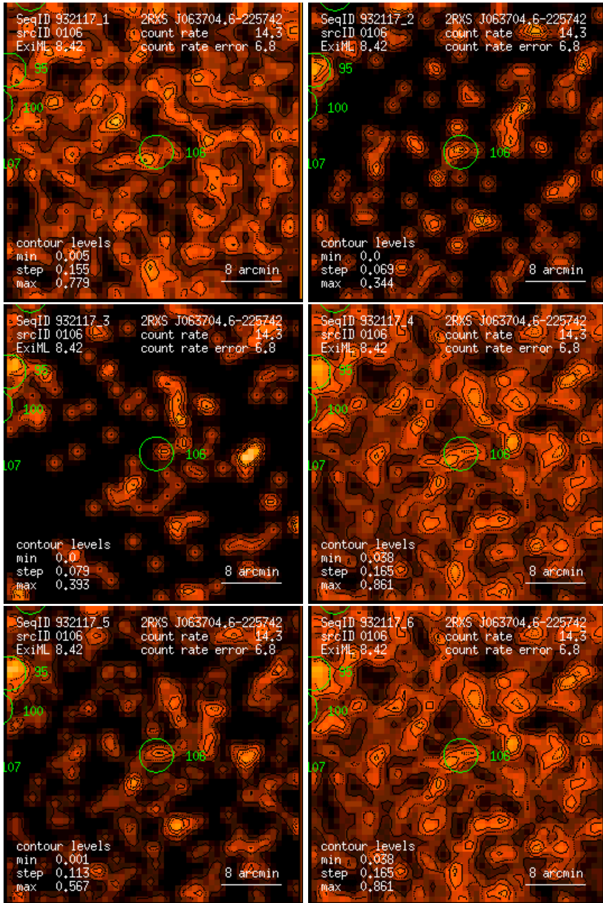
Figure 106: RASS 932117: detection 0106: band rate images, Gaussian filter: (1) PSPC channels 11 – 41, (2) 52 – 90, (3) 91 – 201, (4) 11 – 235, (5) 52 – 201, (6) 11 – 201. Broad band rates in counts/ks. Band rate contour levels in counts/ks/arcmin 2 .
