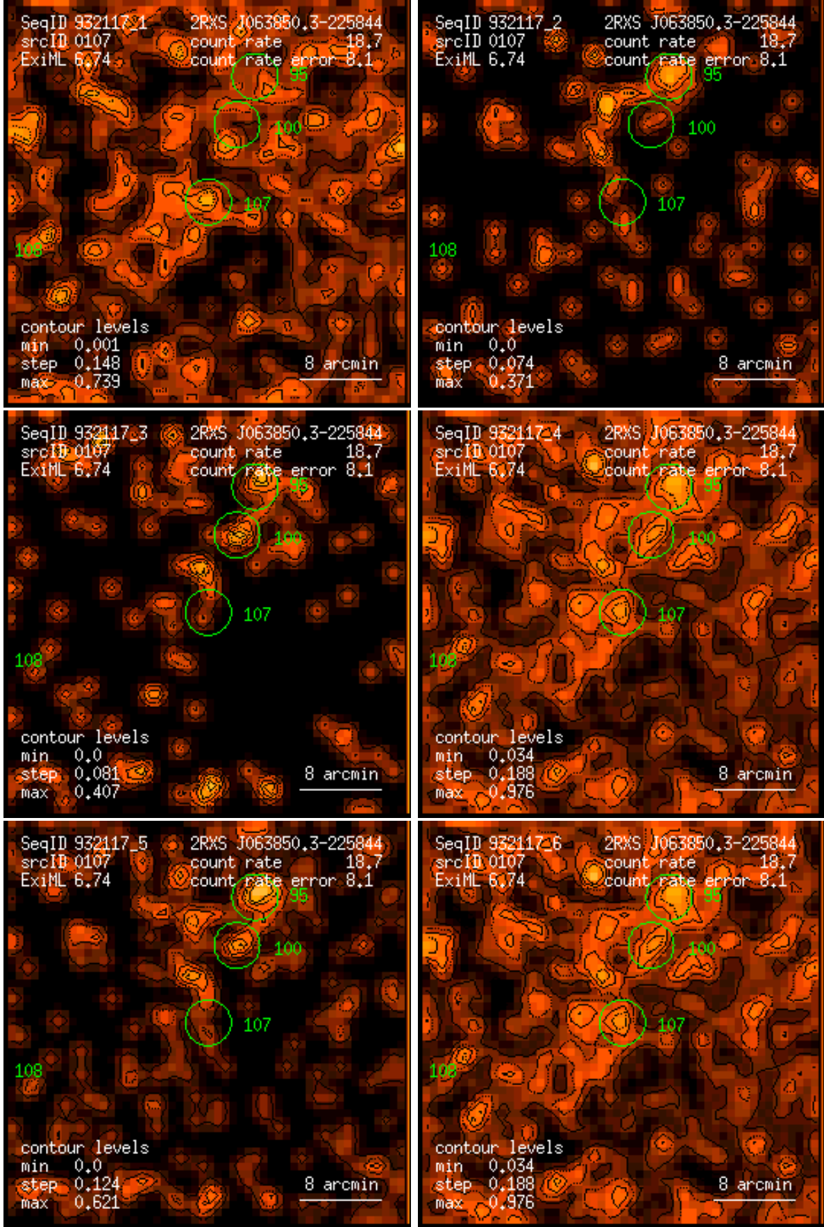
Figure 107: RASS 932117: detection 0107: band rate images, Gaussian filter: (1) PSPC channels 11 – 41, (2) 52 – 90, (3) 91 – 201, (4) 11 – 235, (5) 52 – 201, (6) 11 – 201. Broad band rates in counts/ks. Band rate contour levels in counts/ks/arcmin 2 .
