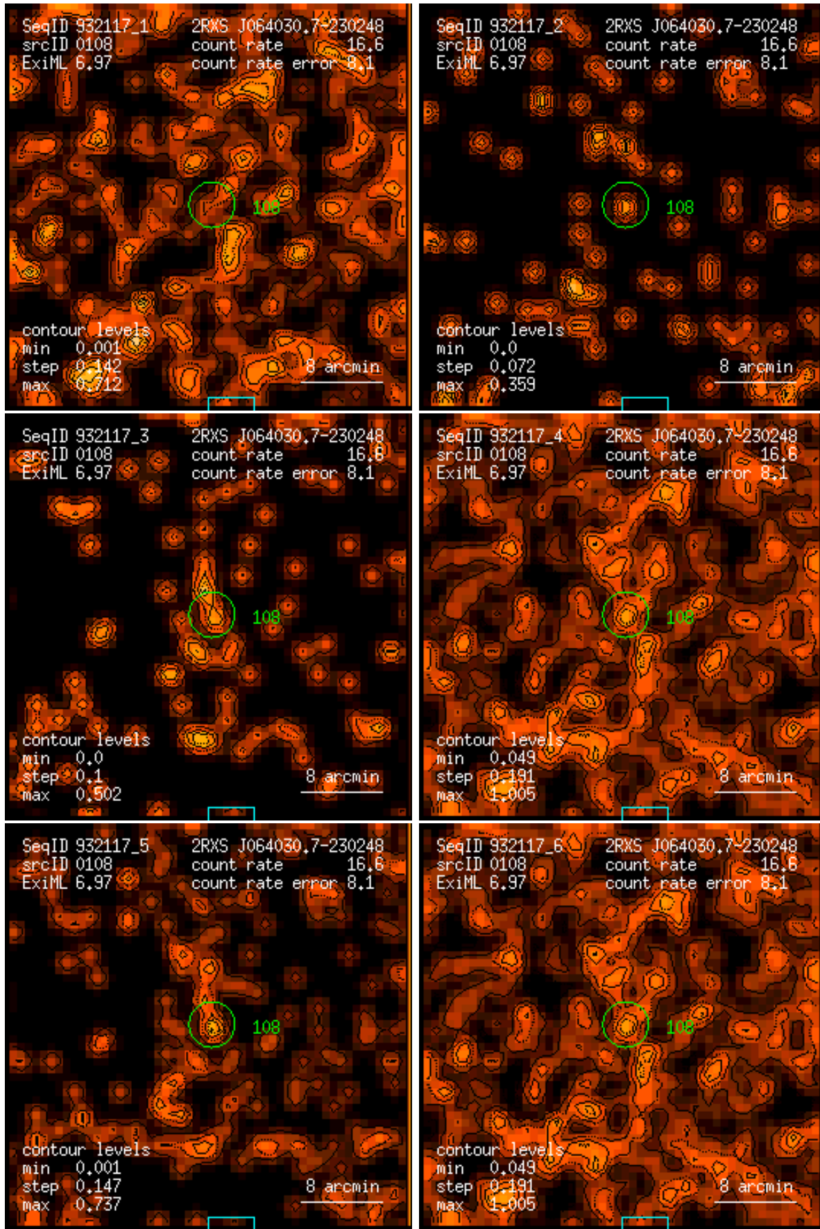
Figure 108: RASS 932117: detection 0108: band rate images, Gaussian filter: (1) PSPC channels 11 – 41, (2) 52 – 90, (3) 91 – 201, (4) 11 – 235, (5) 52 – 201, (6) 11 – 201. Broad band rates in counts/ks. Band rate contour levels in counts/ks/arcmin 2 .
