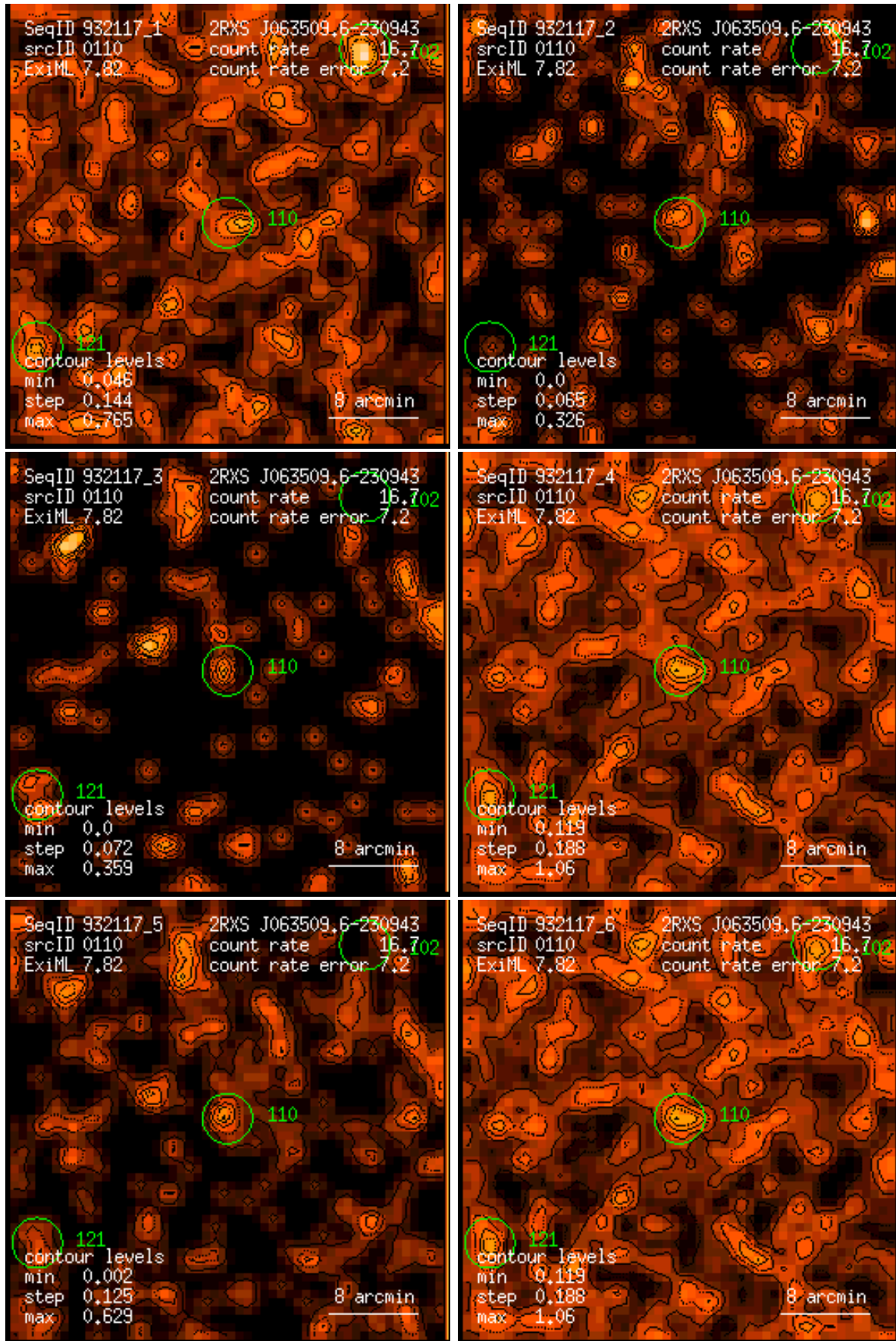
Figure 110: RASS 932117: detection 0110: band rate images, Gaussian filter: (1) PSPC channels 11 – 41, (2) 52 – 90, (3) 91 – 201, (4) 11 – 235, (5) 52 – 201, (6) 11 – 201. Broad band rates in counts/ks. Band rate contour levels in counts/ks/arcmin 2 .
