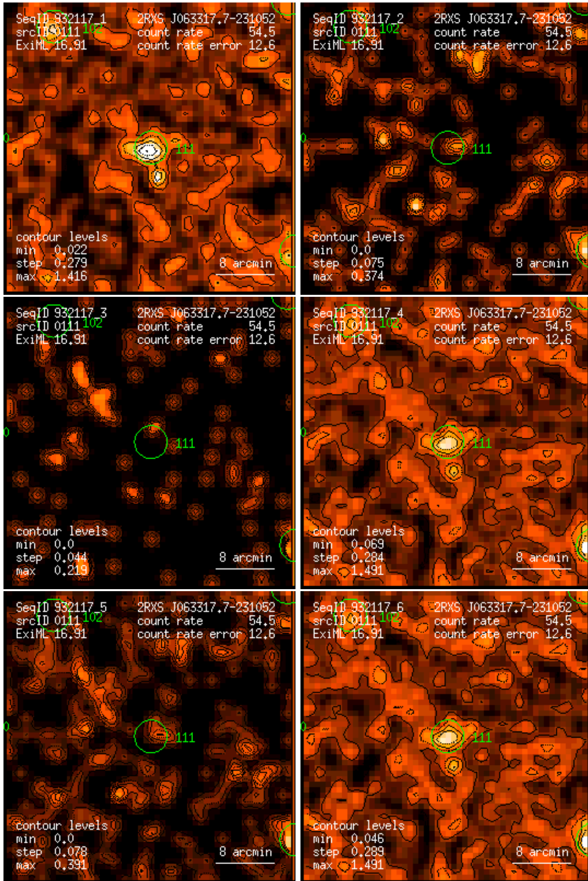
Figure 111: RASS 932117: detection 0111: band rate images, Gaussian filter: (1) PSPC channels 11 – 41, (2) 52 – 90, (3) 91 – 201, (4) 11 – 235, (5) 52 – 201, (6) 11 – 201. Broad band rates in counts/ks. Band rate contour levels in counts/ks/arcmin 2 .
