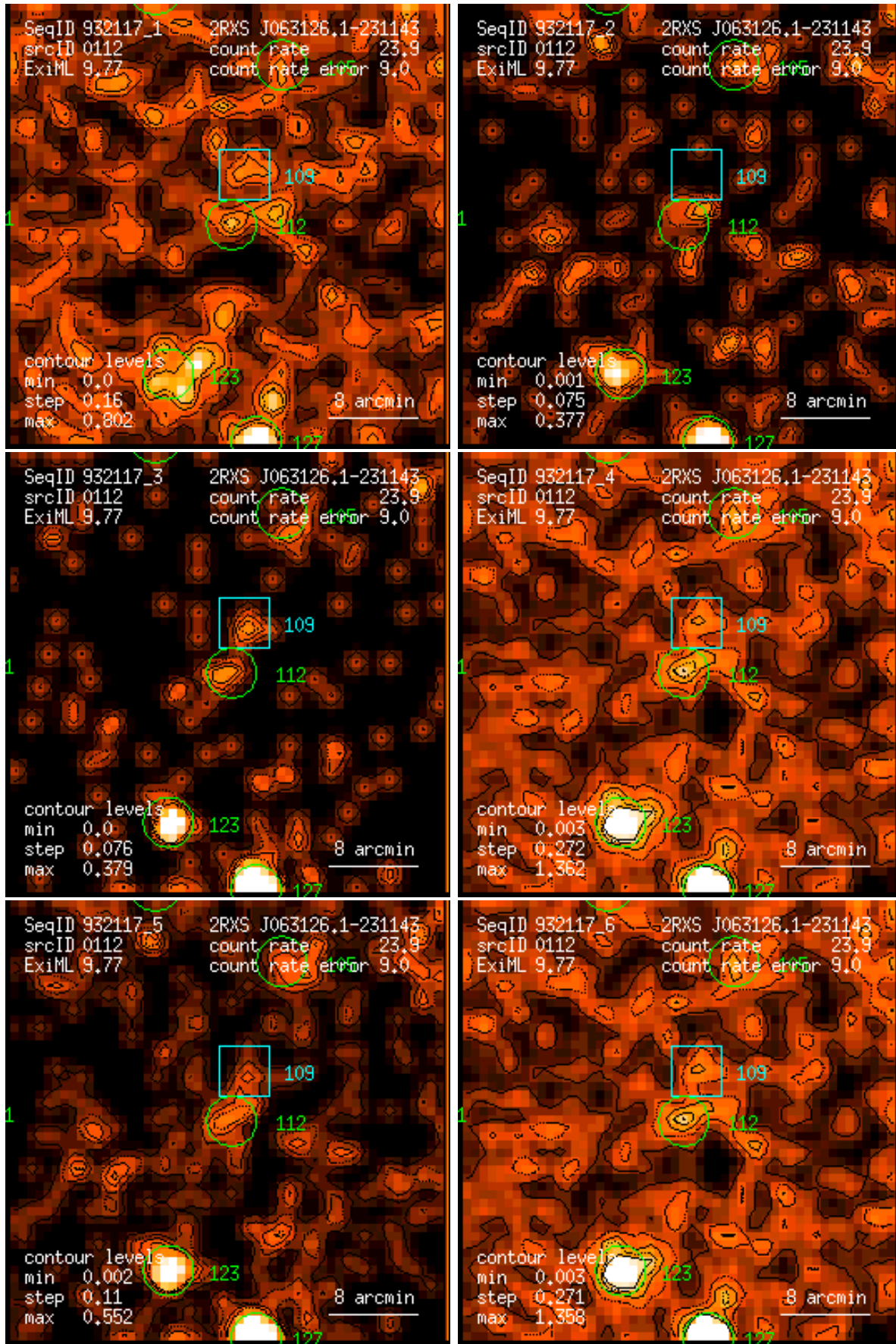
Figure 112: RASS 932117: detection 0112: band rate images, Gaussian filter: (1) PSPC channels 11 – 41, (2) 52 – 90, (3) 91 – 201, (4) 11 – 235, (5) 52 – 201, (6) 11 – 201. Broad band rates in counts/ks. Band rate contour levels in counts/ks/arcmin 2 .
