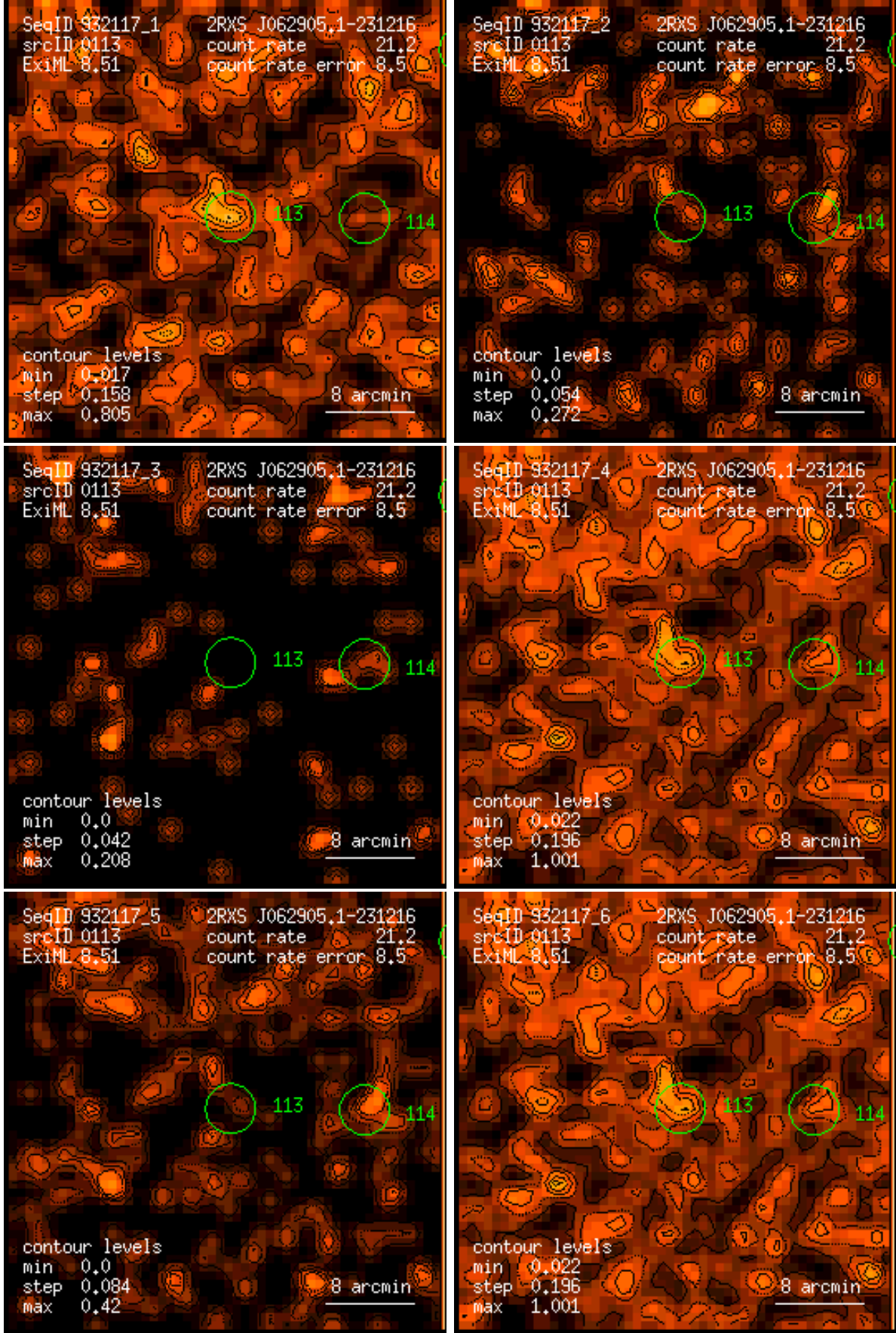
Figure 113: RASS 932117: detection 0113: band rate images, Gaussian filter: (1) PSPC channels 11 – 41, (2) 52 – 90, (3) 91 – 201, (4) 11 – 235, (5) 52 – 201, (6) 11 – 201. Broad band rates in counts/ks. Band rate contour levels in counts/ks/arcmin 2 .
