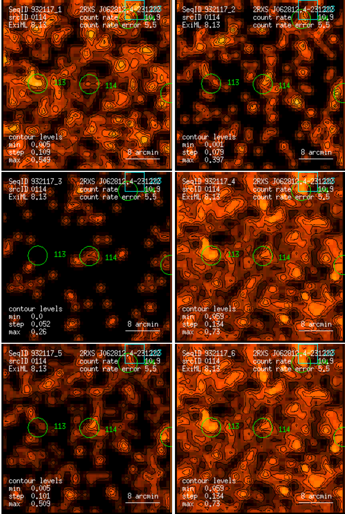
Figure 114: RASS 932117: detection 0114: band rate images, Gaussian filter: (1) PSPC channels 11 – 41, (2) 52 – 90, (3) 91 – 201, (4) 11 – 235, (5) 52 – 201, (6) 11 – 201. Broad band rates in counts/ks. Band rate contour levels in counts/ks/arcmin 2 .
