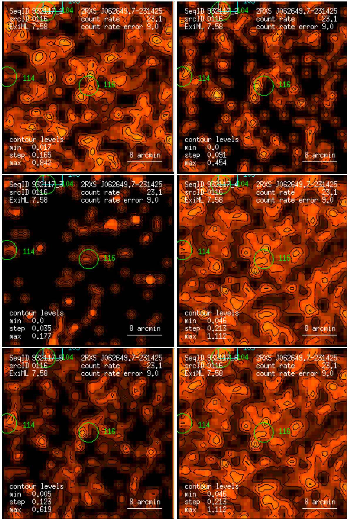
Figure 116: RASS 932117: detection 0116: band rate images, Gaussian filter: (1) PSPC channels 11 – 41, (2) 52 – 90, (3) 91 – 201, (4) 11 – 235, (5) 52 – 201, (6) 11 – 201. Broad band rates in counts/ks. Band rate contour levels in counts/ks/arcmin 2 .
