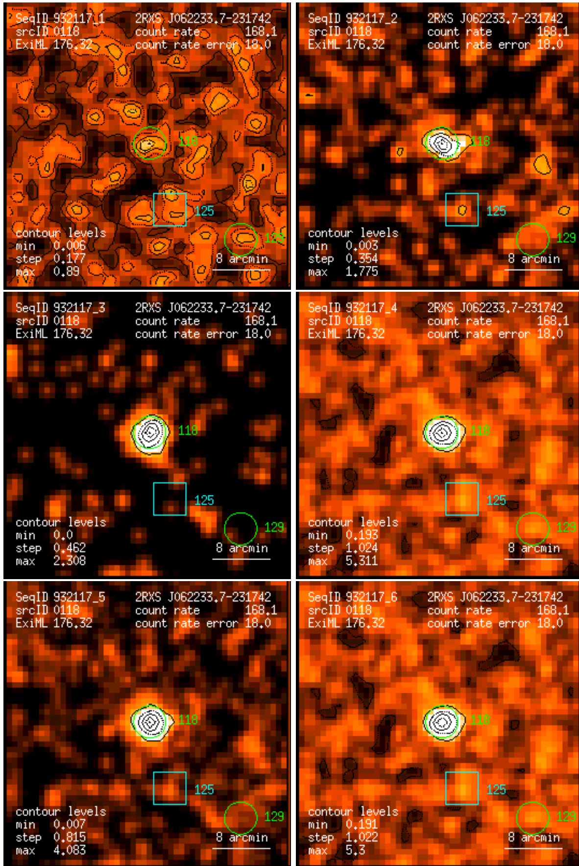
Figure 118: RASS 932117: detection 0118: band rate images, Gaussian filter: (1) PSPC channels 11 – 41, (2) 52 – 90, (3) 91 – 201, (4) 11 – 235, (5) 52 – 201, (6) 11 – 201. Broad band rates in counts/ks. Band rate contour levels in counts/ks/arcmin 2 .
