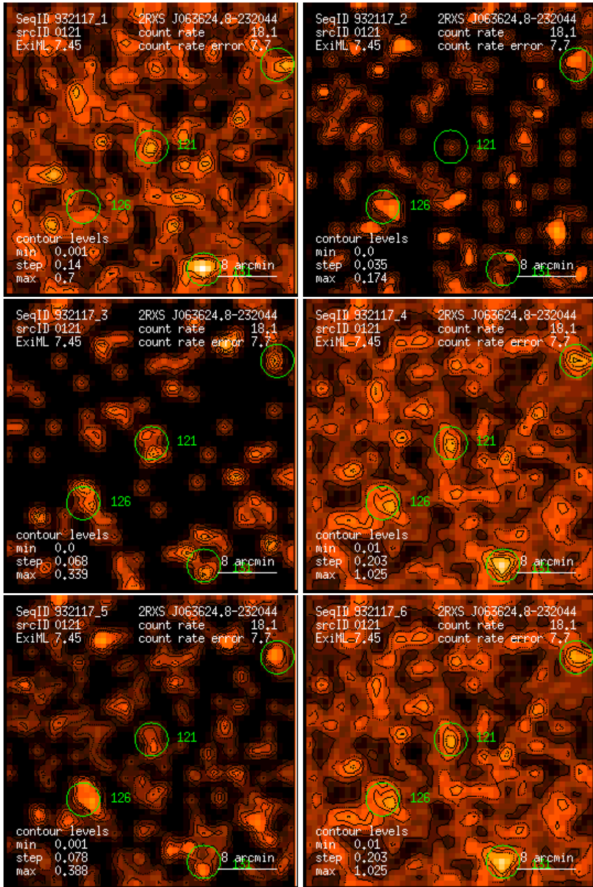
Figure 121: RASS 932117: detection 0121: band rate images, Gaussian filter: (1) PSPC channels 11 – 41, (2) 52 – 90, (3) 91 – 201, (4) 11 – 235, (5) 52 – 201, (6) 11 – 201. Broad band rates in counts/ks. Band rate contour levels in counts/ks/arcmin 2 .
