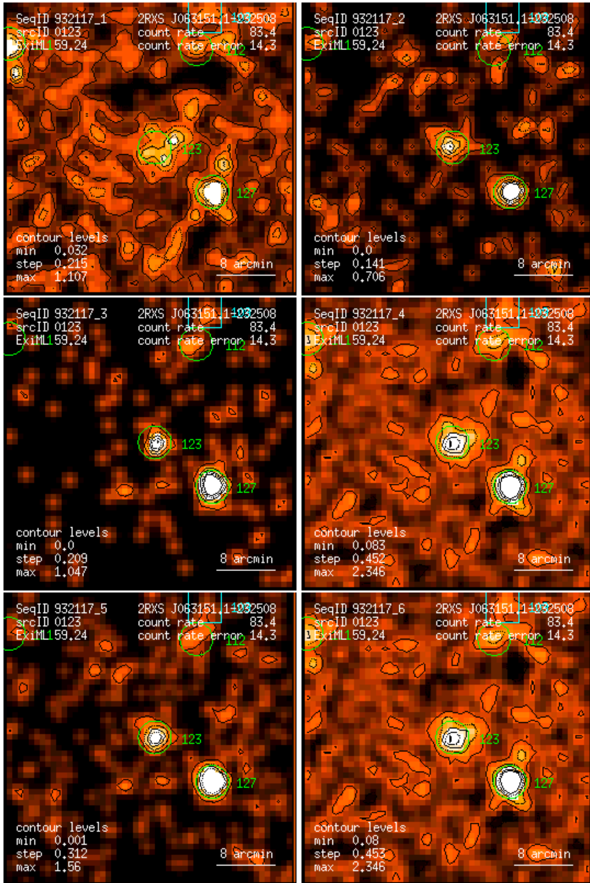
Figure 123: RASS 932117: detection 0123: band rate images, Gaussian filter: (1) PSPC channels 11 – 41, (2) 52 – 90, (3) 91 – 201, (4) 11 – 235, (5) 52 – 201, (6) 11 – 201. Broad band rates in counts/ks. Band rate contour levels in counts/ks/arcmin 2 .
