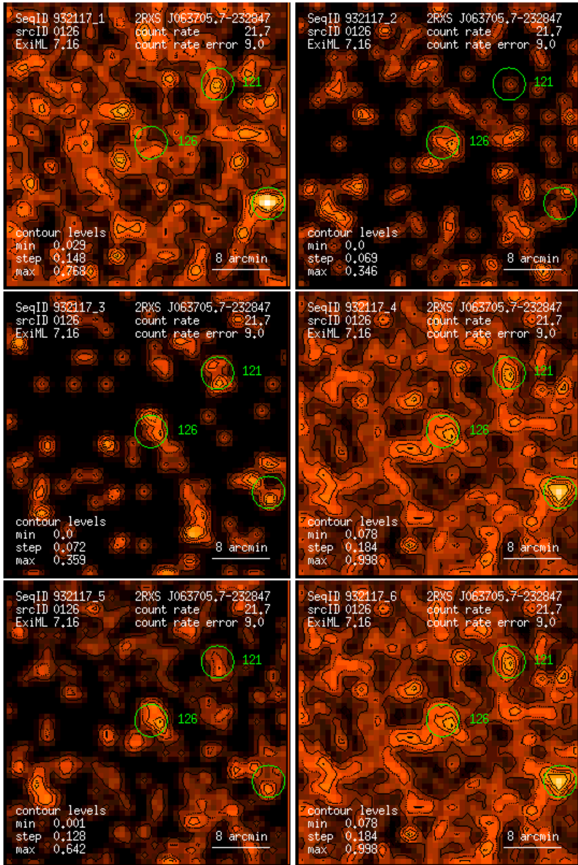
Figure 126: RASS 932117: detection 0126: band rate images, Gaussian filter: (1) PSPC channels 11 – 41, (2) 52 – 90, (3) 91 – 201, (4) 11 – 235, (5) 52 – 201, (6) 11 – 201. Broad band rates in counts/ks. Band rate contour levels in counts/ks/arcmin 2 .
