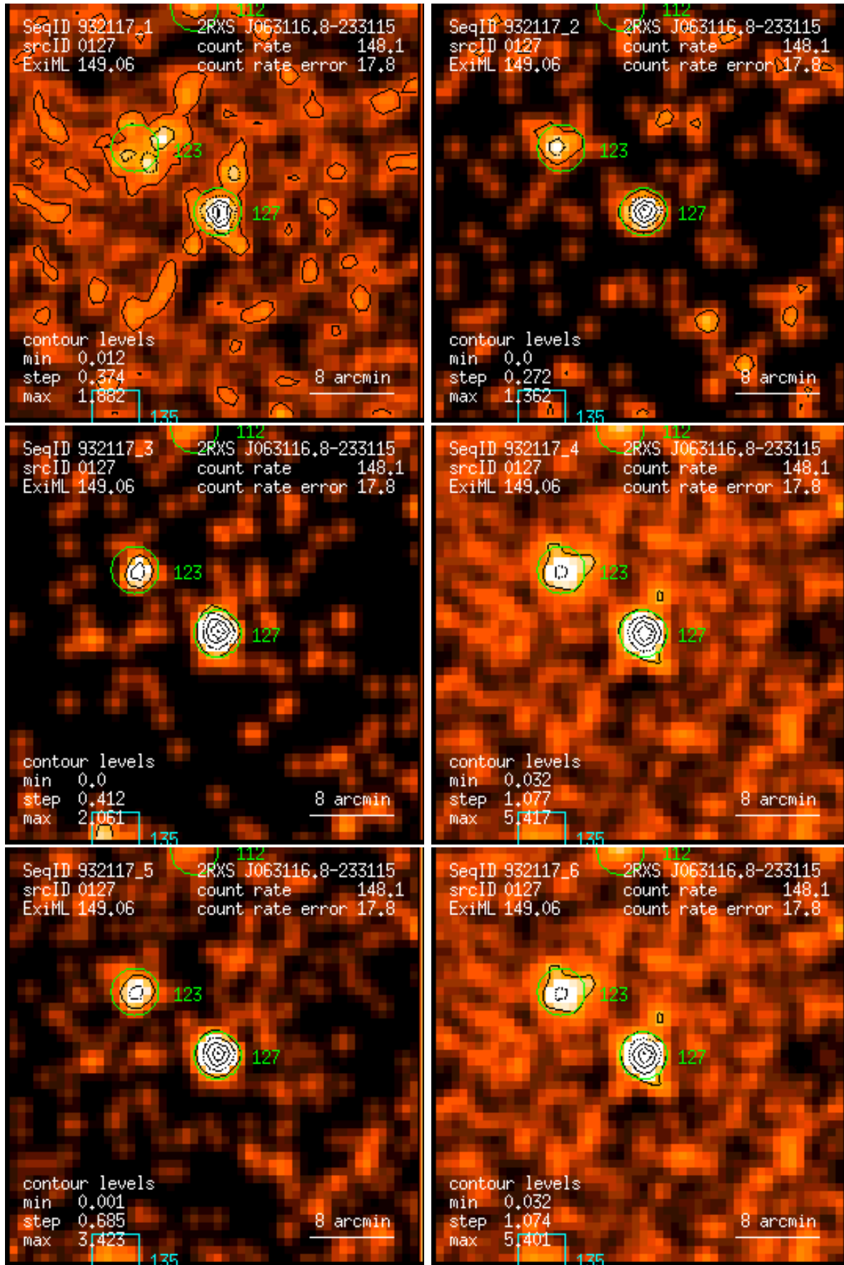
Figure 127: RASS 932117: detection 0127: band rate images, Gaussian filter: (1) PSPC channels 11 – 41, (2) 52 – 90, (3) 91 – 201, (4) 11 – 235, (5) 52 – 201, (6) 11 – 201. Broad band rates in counts/ks. Band rate contour levels in counts/ks/arcmin 2 .
