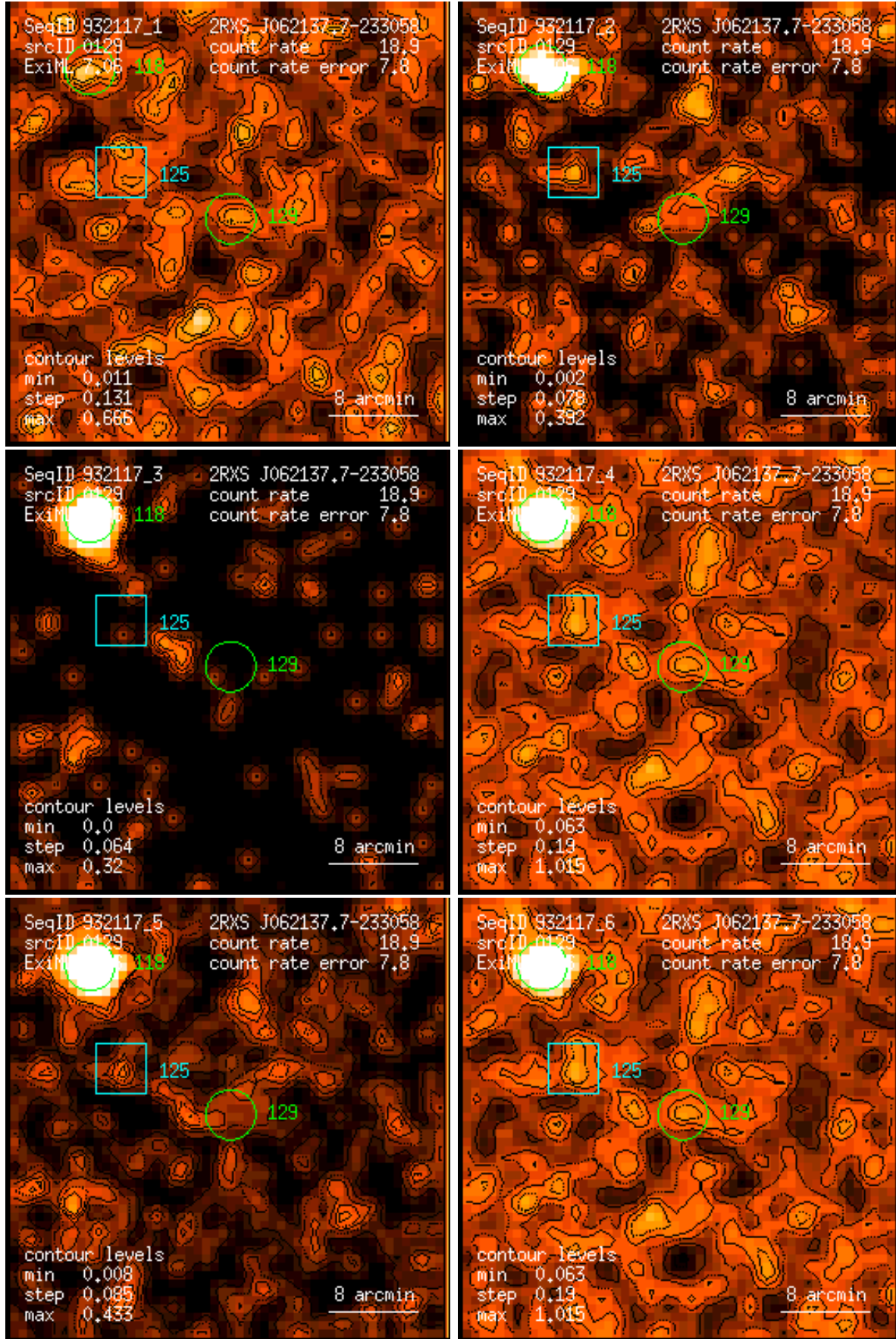
Figure 129: RASS 932117: detection 0129: band rate images, Gaussian filter: (1) PSPC channels 11 – 41, (2) 52 – 90, (3) 91 – 201, (4) 11 – 235, (5) 52 – 201, (6) 11 – 201. Broad band rates in counts/ks. Band rate contour levels in counts/ks/arcmin 2 .
