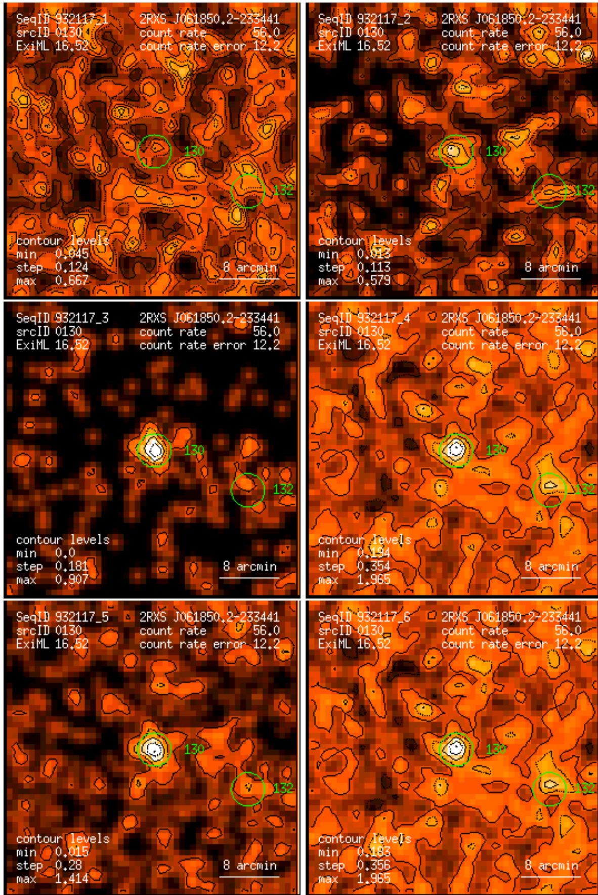
Figure 130: RASS 932117: detection 0130: band rate images, Gaussian filter: (1) PSPC channels 11 – 41, (2) 52 – 90, (3) 91 – 201, (4) 11 – 235, (5) 52 – 201, (6) 11 – 201. Broad band rates in counts/ks. Band rate contour levels in counts/ks/arcmin 2 .
