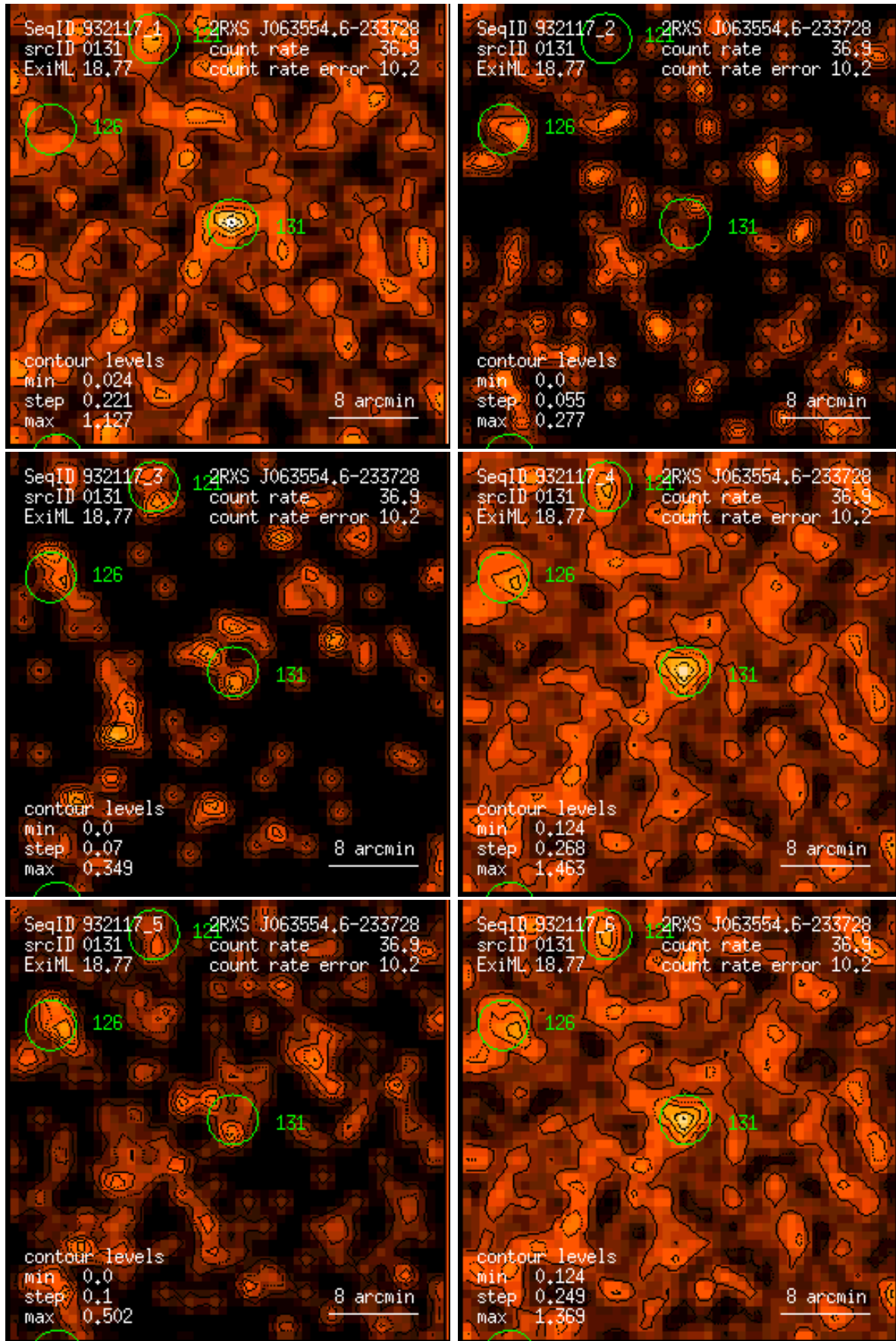
Figure 131: RASS 932117: detection 0131: band rate images, Gaussian filter: (1) PSPC channels 11 – 41, (2) 52 – 90, (3) 91 – 201, (4) 11 – 235, (5) 52 – 201, (6) 11 – 201. Broad band rates in counts/ks. Band rate contour levels in counts/ks/arcmin 2 .
