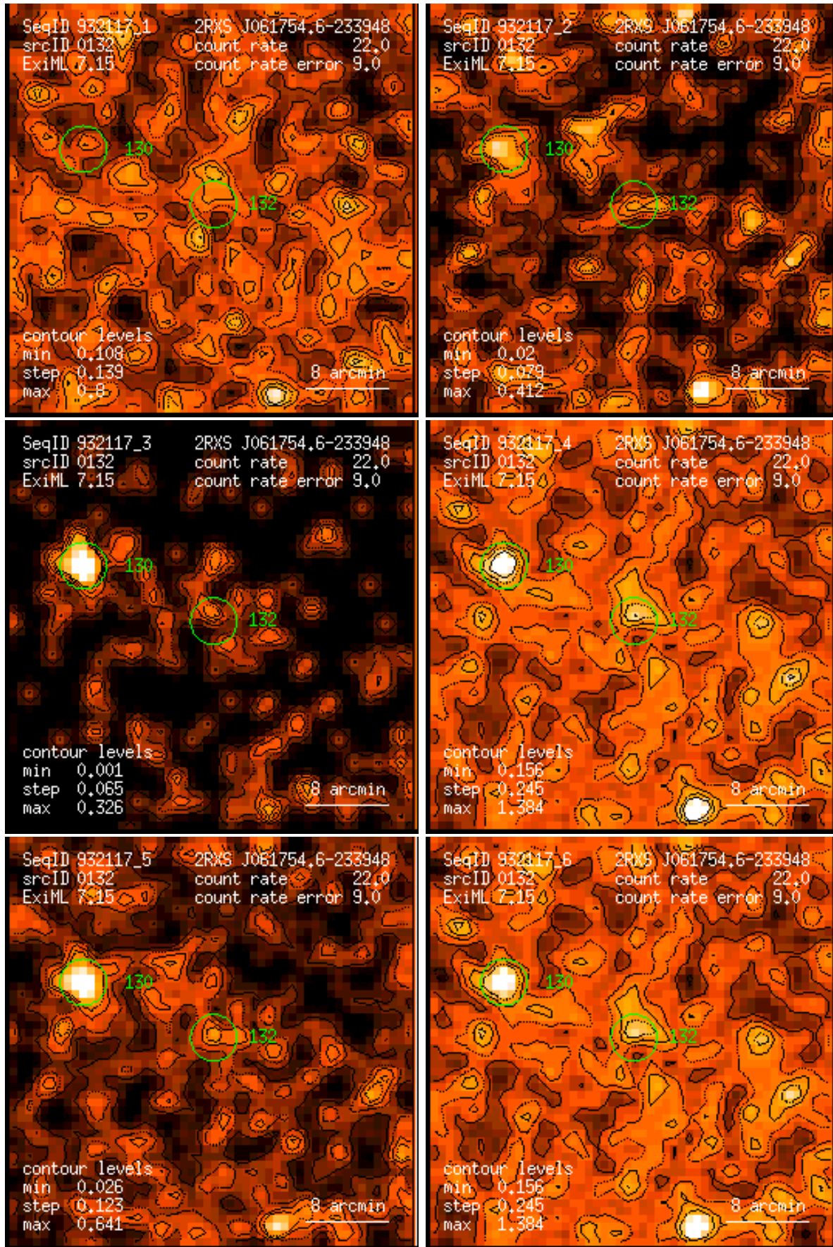
Figure 132: RASS 932117: detection 0132: band rate images, Gaussian filter: (1) PSPC channels 11 – 41, (2) 52 – 90, (3) 91 – 201, (4) 11 – 235, (5) 52 – 201, (6) 11 – 201. Broad band rates in counts/ks. Band rate contour levels in counts/ks/arcmin 2 .
