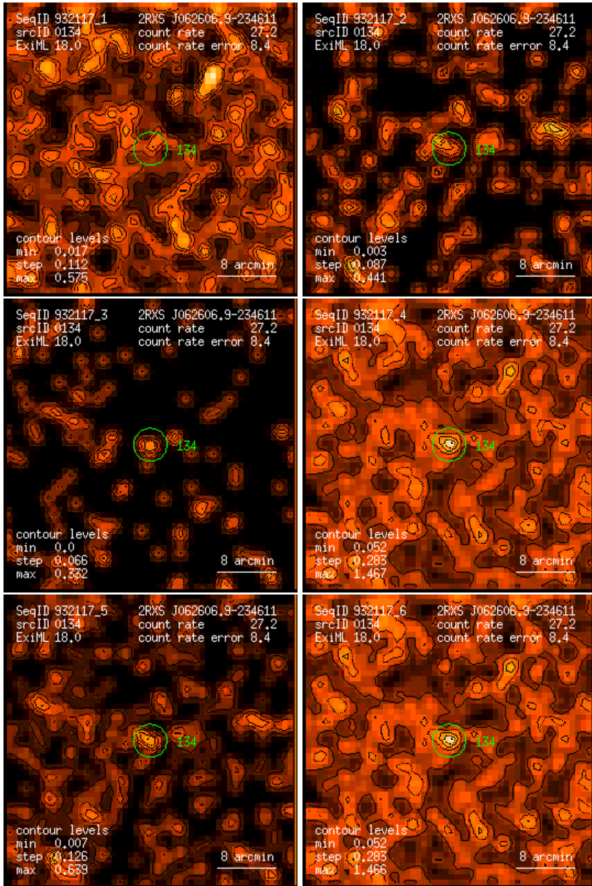
Figure 134: RASS 932117: detection 0134: band rate images, Gaussian filter: (1) PSPC channels 11 – 41, (2) 52 – 90, (3) 91 – 201, (4) 11 – 235, (5) 52 – 201, (6) 11 – 201. Broad band rates in counts/ks. Band rate contour levels in counts/ks/arcmin 2 .
