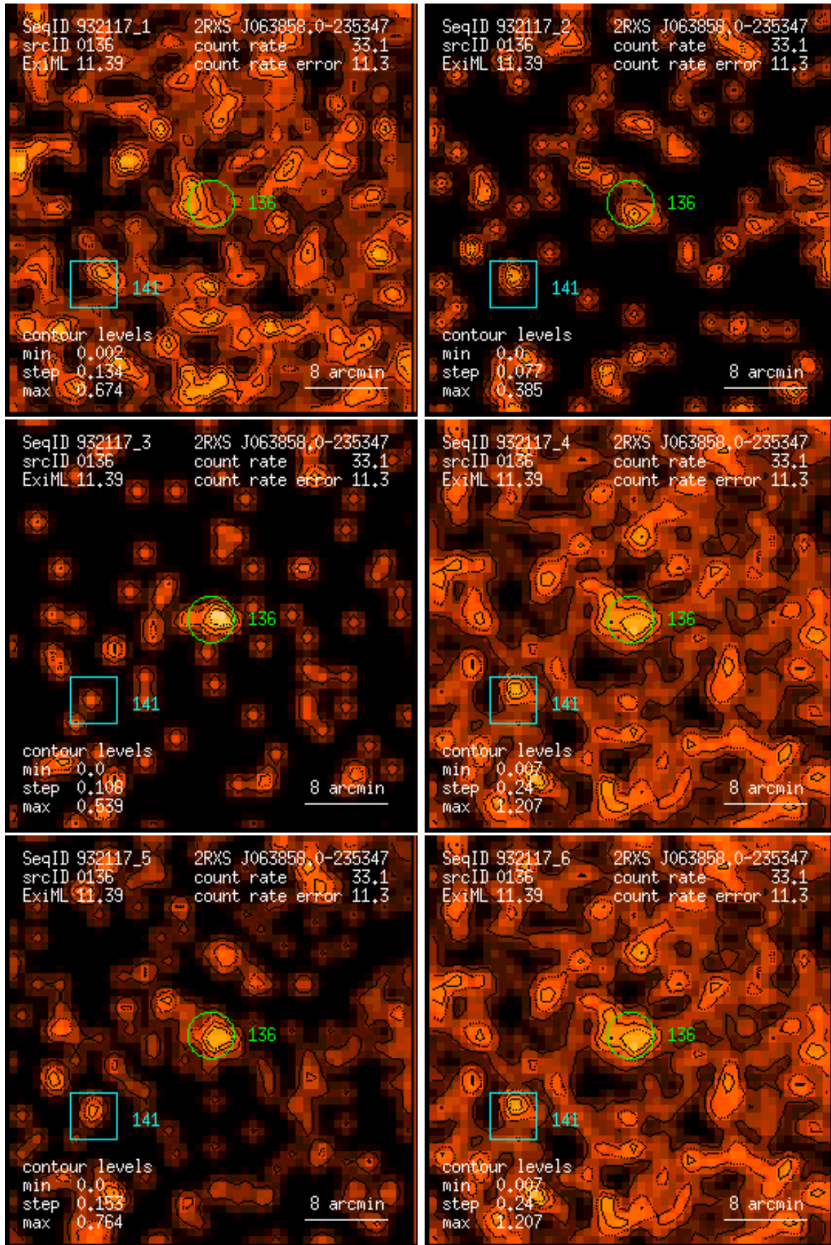
Figure 136: RASS 932117: detection 0136: band rate images, Gaussian filter: (1) PSPC channels 11 – 41, (2) 52 – 90, (3) 91 – 201, (4) 11 – 235, (5) 52 – 201, (6) 11 – 201. Broad band rates in counts/ks. Band rate contour levels in counts/ks/arcmin 2 .
