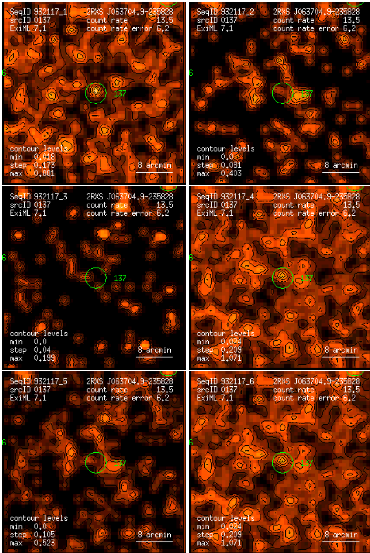
Figure 137: RASS 932117: detection 0137: band rate images, Gaussian filter: (1) PSPC channels 11 – 41, (2) 52 – 90, (3) 91 – 201, (4) 11 – 235, (5) 52 – 201, (6) 11 – 201. Broad band rates in counts/ks. Band rate contour levels in counts/ks/arcmin 2 .
