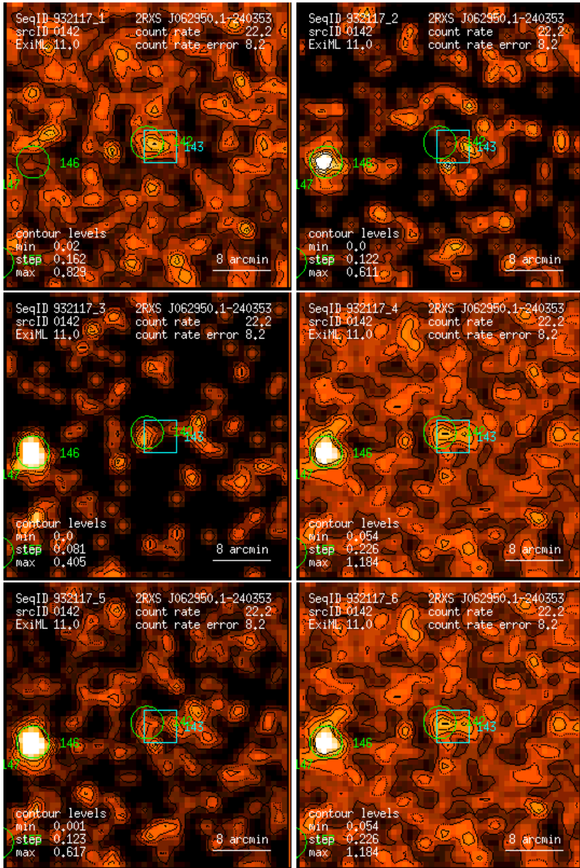
Figure 142: RASS 932117: detection 0142: band rate images, Gaussian filter: (1) PSPC channels 11 – 41, (2) 52 – 90, (3) 91 – 201, (4) 11 – 235, (5) 52 – 201, (6) 11 – 201. Broad band rates in counts/ks. Band rate contour levels in counts/ks/arcmin 2 .
