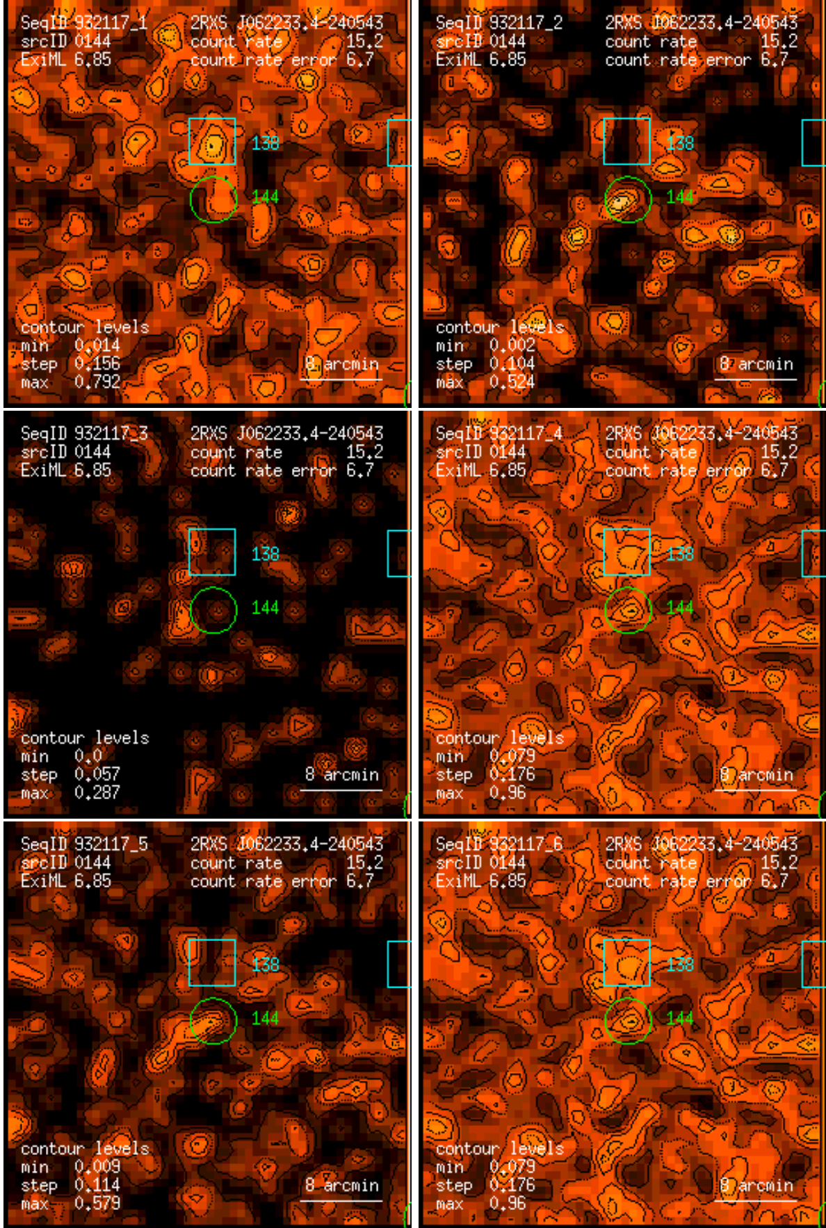
Figure 144: RASS 932117: detection 0144: band rate images, Gaussian filter: (1) PSPC channels 11 – 41, (2) 52 – 90, (3) 91 – 201, (4) 11 – 235, (5) 52 – 201, (6) 11 – 201. Broad band rates in counts/ks. Band rate contour levels in counts/ks/arcmin 2 .
