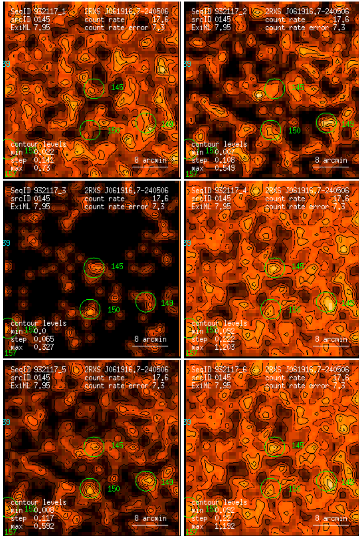
Figure 145: RASS 932117: detection 0145: band rate images, Gaussian filter: (1) PSPC channels 11 – 41, (2) 52 – 90, (3) 91 – 201, (4) 11 – 235, (5) 52 – 201, (6) 11 – 201. Broad band rates in counts/ks. Band rate contour levels in counts/ks/arcmin 2 .
