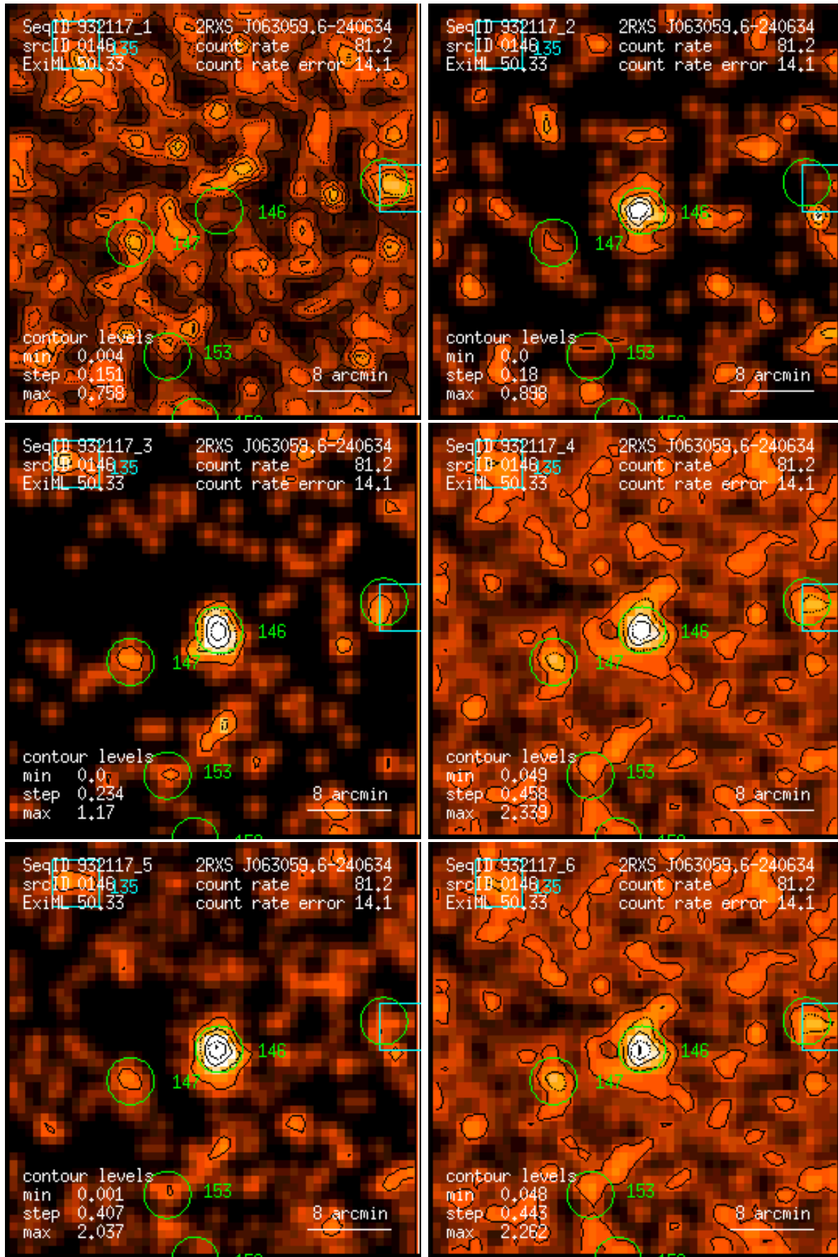
Figure 146: RASS 932117: detection 0146: band rate images, Gaussian filter: (1) PSPC channels 11 – 41, (2) 52 – 90, (3) 91 – 201, (4) 11 – 235, (5) 52 – 201, (6) 11 – 201. Broad band rates in counts/ks. Band rate contour levels in counts/ks/arcmin 2 .
