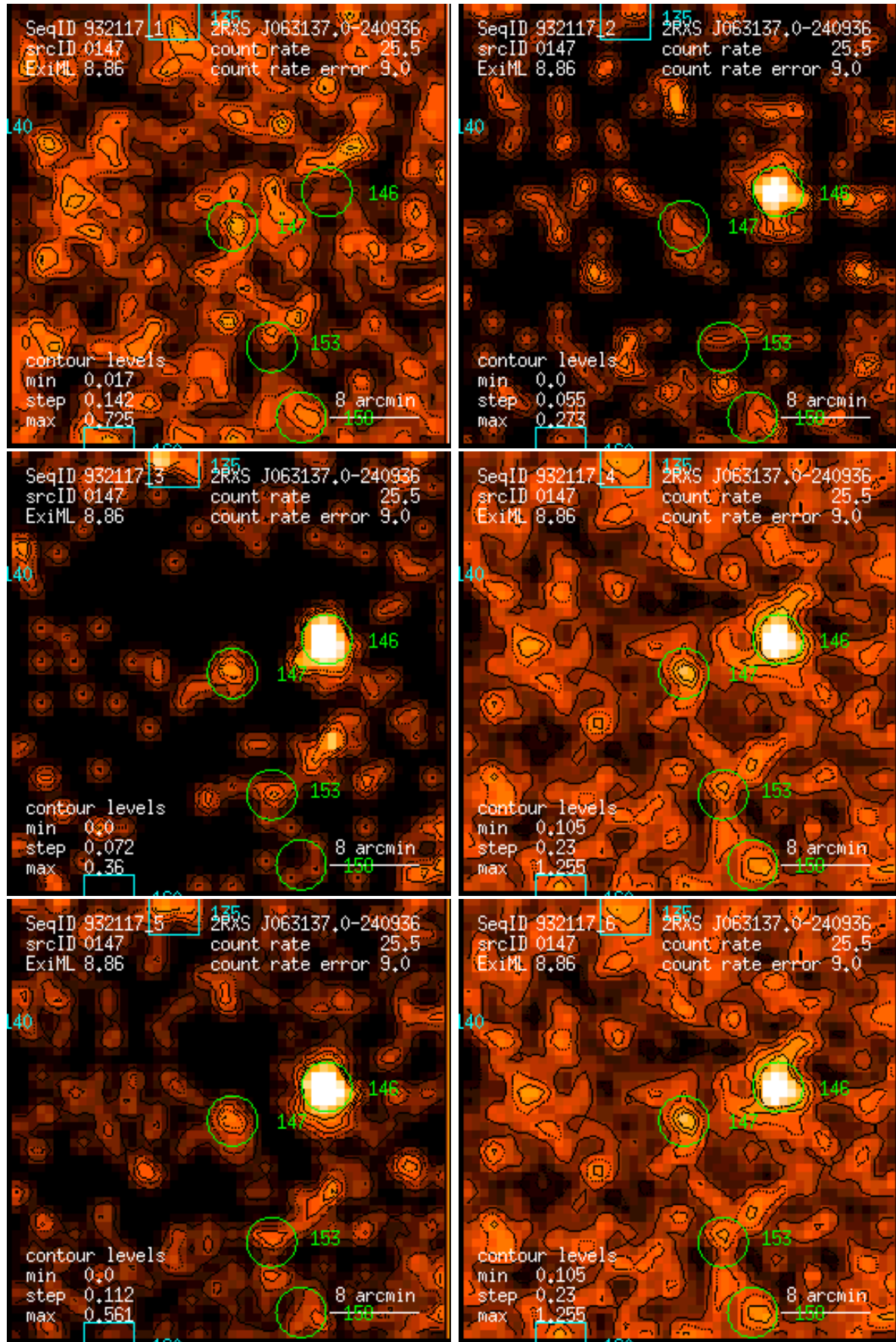
Figure 147: RASS 932117: detection 0147: band rate images, Gaussian filter: (1) PSPC channels 11 – 41, (2) 52 – 90, (3) 91 – 201, (4) 11 – 235, (5) 52 – 201, (6) 11 – 201. Broad band rates in counts/ks. Band rate contour levels in counts/ks/arcmin 2 .
