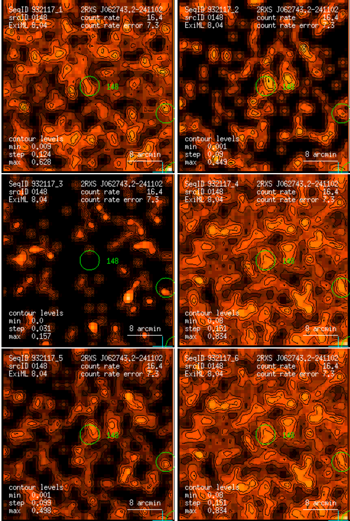
Figure 148: RASS 932117: detection 0148: band rate images, Gaussian filter: (1) PSPC channels 11 – 41, (2) 52 – 90, (3) 91 – 201, (4) 11 – 235, (5) 52 – 201, (6) 11 – 201. Broad band rates in counts/ks. Band rate contour levels in counts/ks/arcmin 2 .
