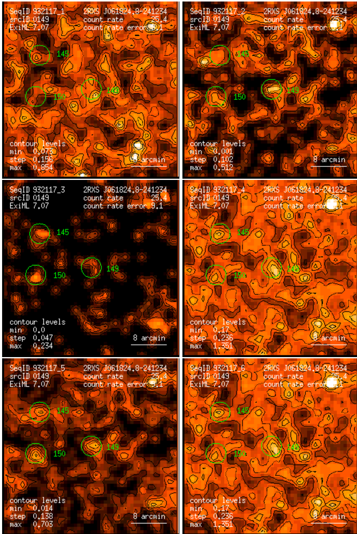
Figure 149: RASS 932117: detection 0149: band rate images, Gaussian filter: (1) PSPC channels 11 – 41, (2) 52 – 90, (3) 91 – 201, (4) 11 – 235, (5) 52 – 201, (6) 11 – 201. Broad band rates in counts/ks. Band rate contour levels in counts/ks/arcmin 2 .
