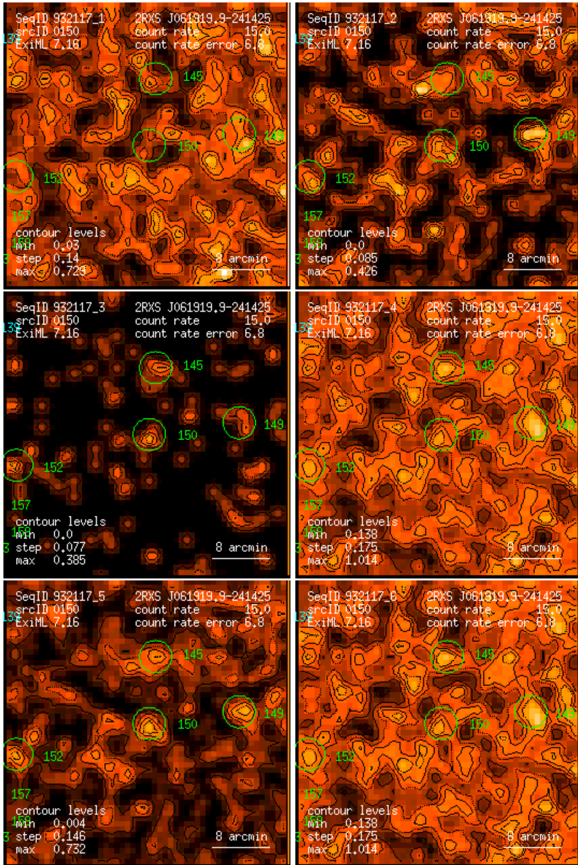
Figure 150: RASS 932117: detection 0150: band rate images, Gaussian filter: (1) PSPC channels 11 – 41, (2) 52 – 90, (3) 91 – 201, (4) 11 – 235, (5) 52 – 201, (6) 11 – 201. Broad band rates in counts/ks. Band rate contour levels in counts/ks/arcmin 2 .
