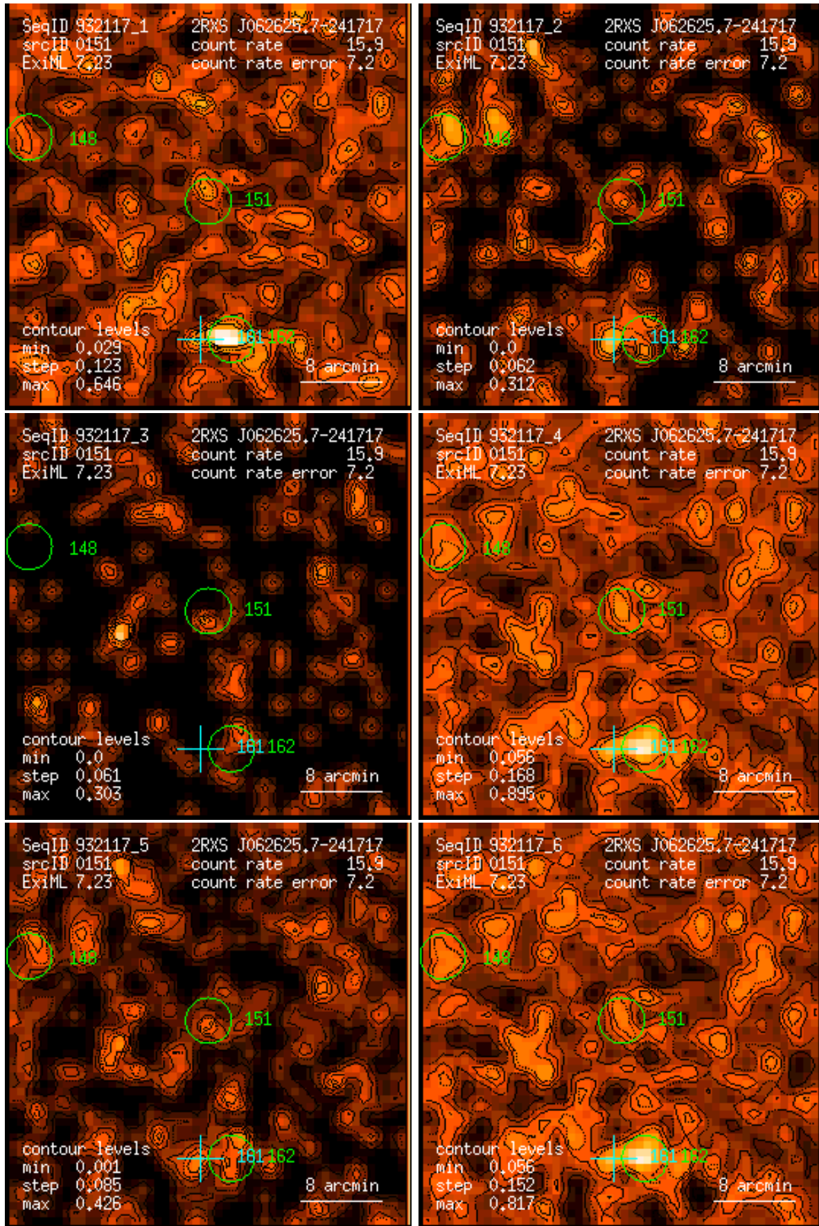
Figure 151: RASS 932117: detection 0151: band rate images, Gaussian filter: (1) PSPC channels 11 – 41, (2) 52 – 90, (3) 91 – 201, (4) 11 – 235, (5) 52 – 201, (6) 11 – 201. Broad band rates in counts/ks. Band rate contour levels in counts/ks/arcmin 2 .
