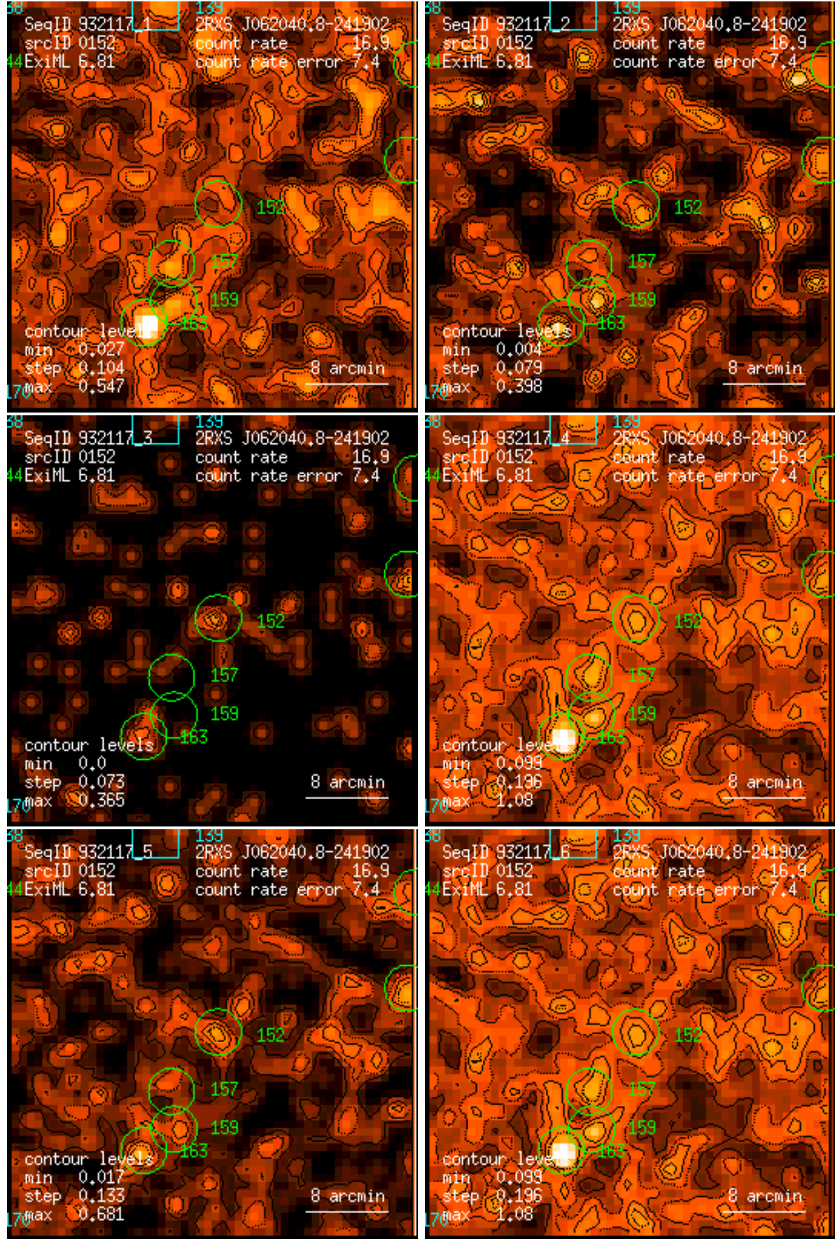
Figure 152: RASS 932117: detection 0152: band rate images, Gaussian filter: (1) PSPC channels 11 – 41, (2) 52 – 90, (3) 91 – 201, (4) 11 – 235, (5) 52 – 201, (6) 11 – 201. Broad band rates in counts/ks. Band rate contour levels in counts/ks/arcmin 2 .
