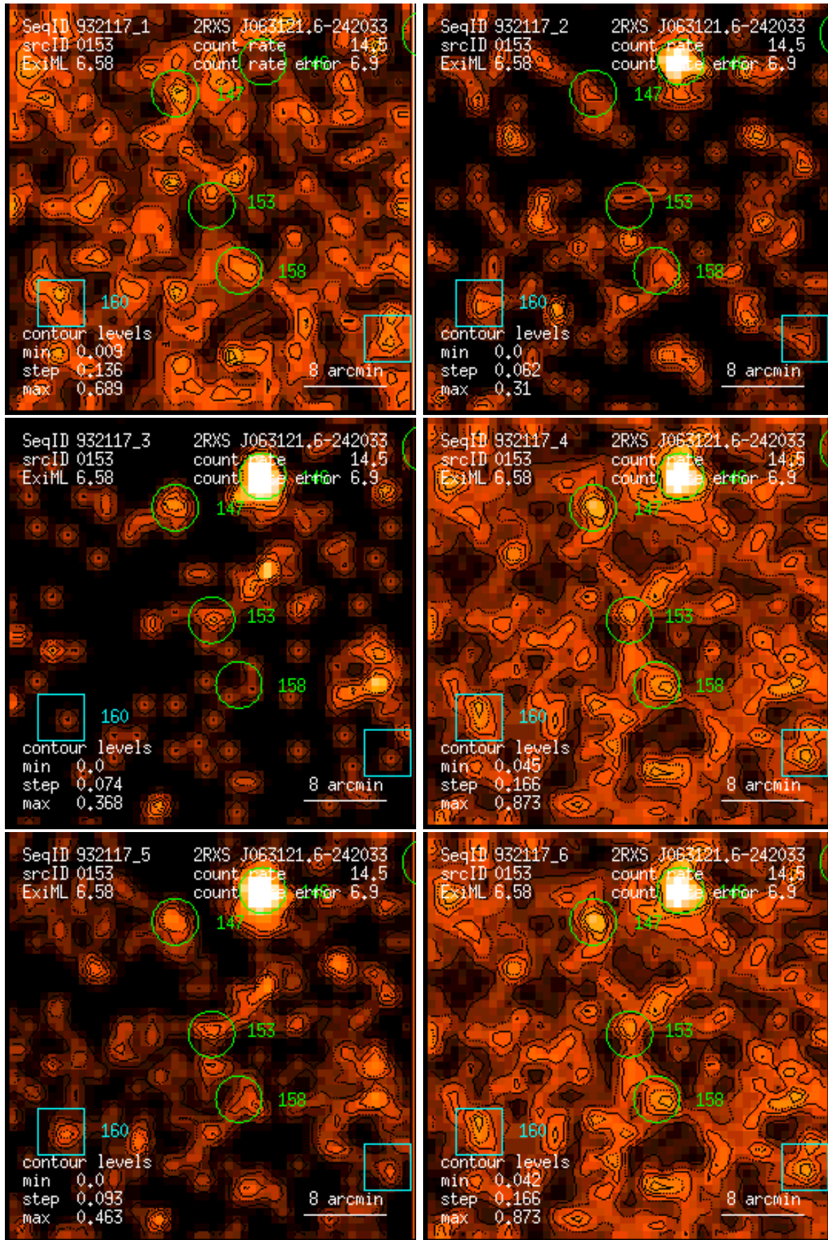
Figure 153: RASS 932117: detection 0153: band rate images, Gaussian filter: (1) PSPC channels 11 – 41, (2) 52 – 90, (3) 91 – 201, (4) 11 – 235, (5) 52 – 201, (6) 11 – 201. Broad band rates in counts/ks. Band rate contour levels in counts/ks/arcmin 2 .
